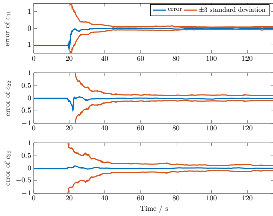
Fig. 7. Estimation errors of the diagonal elements of calibration matrix \mathbf{C} when the data of the first magnetometer axis is scaled by a factor of two. The errors are shown in blue and in red three times the standard deviation estimated by SLAC is shown.
