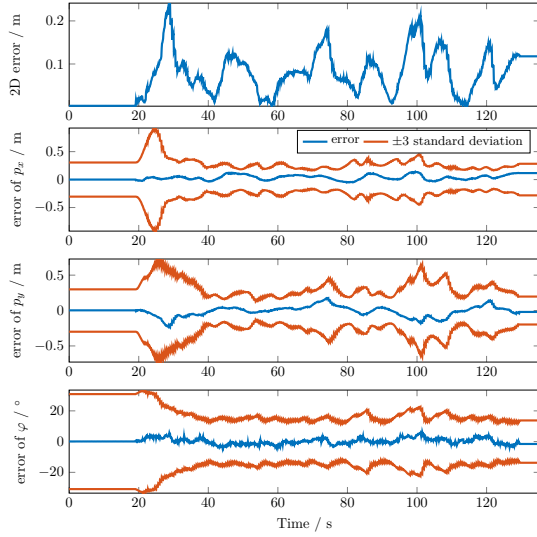
Fig. 3. Position and heading errors over time for trajectory one. The errors are indicated by a blue line and for the lower three plots the red lines show three times the standard deviation of this errors estimated by the Rao-Blackwellized particle filter.
