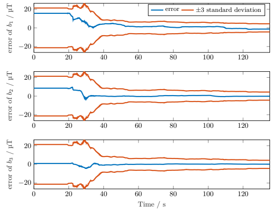
Fig. 6. Estimation error of the bias vector when the data of the first magnetometer axis is scaled by a factor of two. The errors are shown in blue and in red three times the standard deviation estimated by SLAC is shown.
