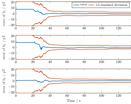
Fig. 4. Estimation error of the bias vector \mathbf{b} = [b_1 \ b_2 \ b_3]^T . The errors are shown in blue and in red three times the standard deviation estimated by SLAC is shown.
