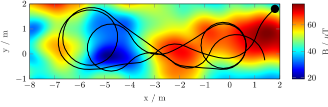
Fig. 1. Magnitude of the magnetic flux density in DLR's laboratory and the trajectory of the first measurement run. The black dot marks the start position of the robot.
