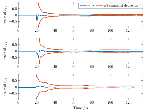
Fig. 5. Estimation errors of the diagonal elements of calibration matrix \mathbf{C} . The errors are shown in blue and in red three times the standard deviation estimated by SLAC is shown.
