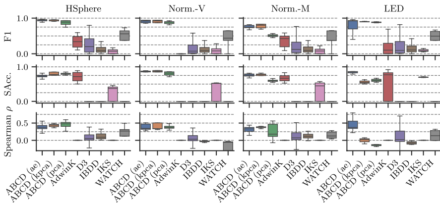
Fig. 3 Results for evaluating change subspace and severity
