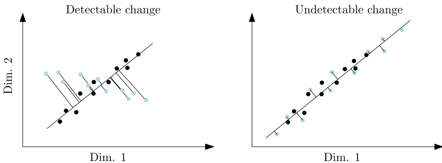
Fig. 6 Illustration of detectable and undetectable change using PCA
