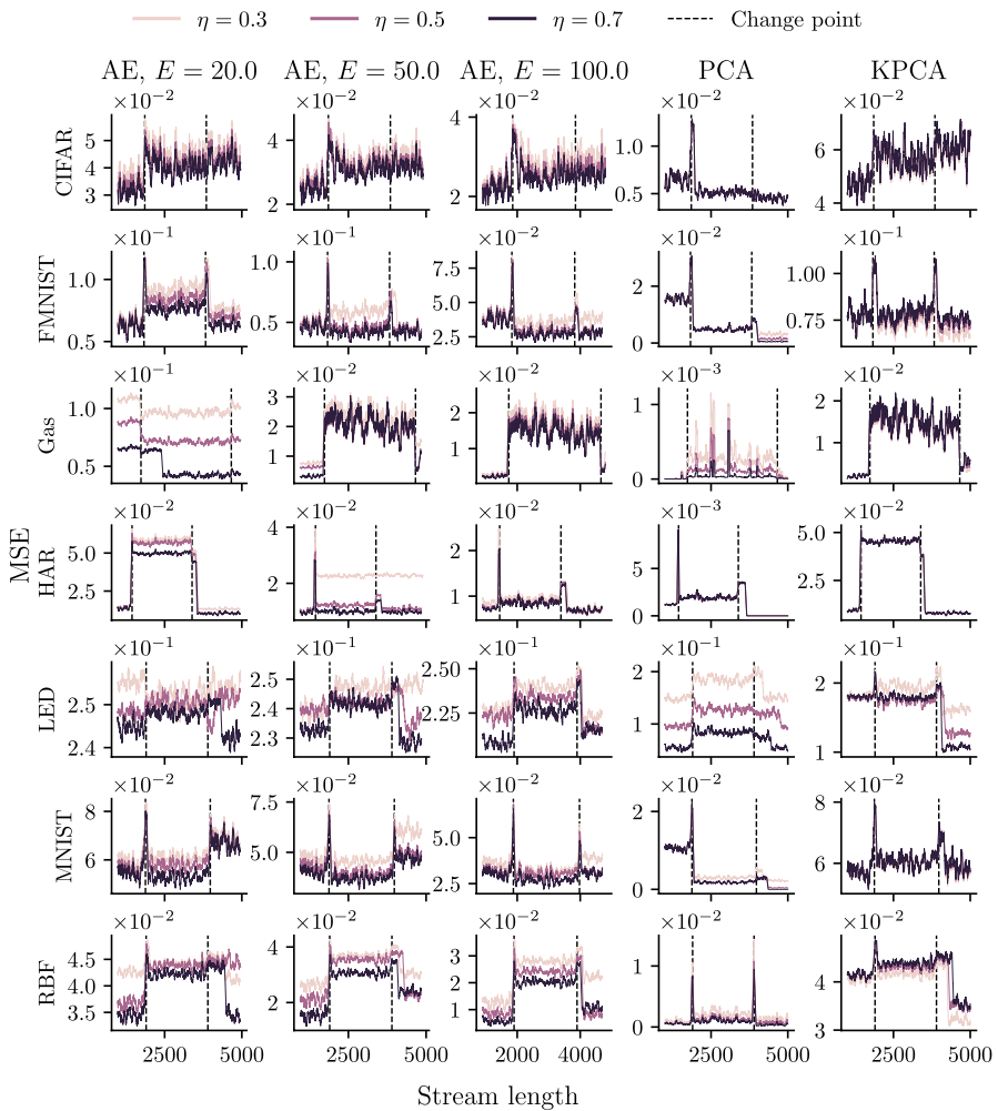
Fig. 7 Reconstruction loss over the length of the stream
