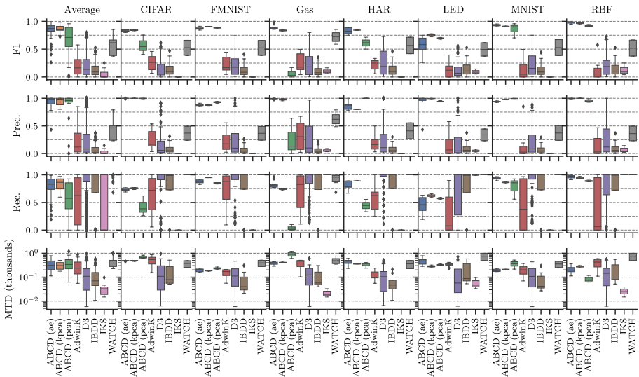
Fig. 2 Change point detection: results for different algorithms and datasets; each box contains the results for the evaluated grid of parameters
