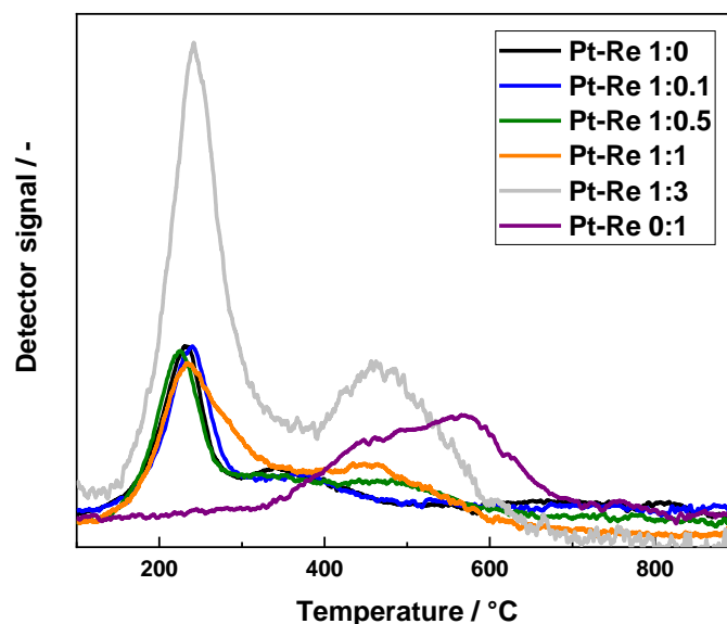
Figure 2: Temperature-programmed reduction of as-prepared bimetallic Pt-Re/Al 2 O 3 catalysts and the monometallic references. Analysis parameters: 10% H 2 /Ar, 10 °C min -1 .
