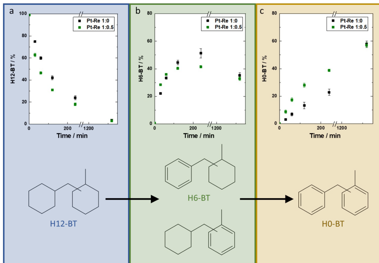
Figure 11: (a) Fraction of H12-BT and (b) build-up of formed H6-BT as well as (c) H0-BT during H_2 release from H12-BT using monometallic Pt-Re 1:0 and bimetallic Pt-Re 1:0.5 catalysts together with the reaction sequence of the dehydrogenation. Reaction conditions: 250 °C, 1 atm, 0.0001 \text{ mol}_{\text{Pt}} \text{ mol}^{-1}_{\text{LOHC}} , 31.01 \text{ g}_{\text{H12-BT}} , 0.30 wt.% Pt, 0 or 0.15 wt.% Re, 1320 min, 300 \text{ mL}_{\text{Ar}} \text{ min}^{-1} .
