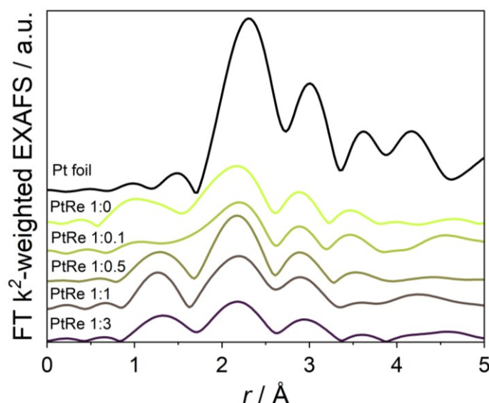
Figure 5: Fourier-transformed EXAFS spectra (Pt L 3 edge, k 2 -weighted) of the bimetallic Pt-Re catalysts with various ratios after reduction at 400 °C for 30 min with 10 °C min -1 in 11% H 2 /He. Spectra were acquired after cool-down to room temperature in 11% H 2 /He.
