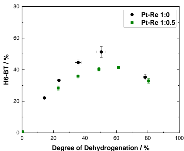
Figure 12: Relationship between the concentration of H6-BT and the degree of dehydrogenation during H_2 release from H12-BT using monometallic Pt-Re 1:0 and bimetallic Pt-Re 1:0.5 catalysts. Reaction conditions: 250 °C, 1 atm, 0.0001 \text{ mol}_{\text{Pt}} \text{ mol}^{-1}_{\text{LOHC}} , 31.01 \text{ g}_{\text{H12-BT}} , 0.30 wt.% Pt, 0 or 0.15 wt.% Re, 1320 min, 300 \text{ mL}_{\text{Ar}} \text{ min}^{-1} .
