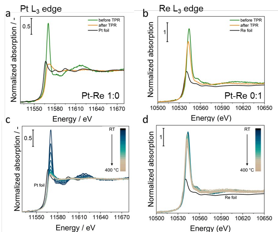
Figure 3: Comparison of in situ X-ray absorption near edge spectra at the Pt and Re L 3 edge acquired at room temperature before and after reduction of (a) the monometallic Pt-Re 1:0 and (b) Pt-Re 0:1 reference catalysts in 11% H 2 /He together with a spectrum for Pt foil, as well as (c,d) in situ spectra during reduction at 400 °C for 30 min with 10 °C min -1 .
