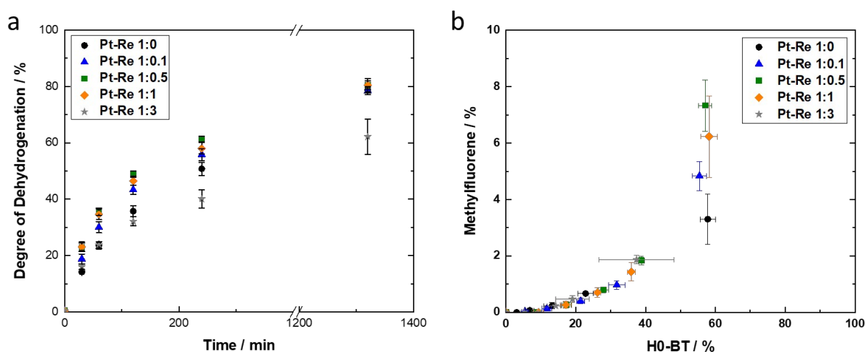
Figure 6: (a) Degree of dehydrogenation and (b) production of methylfluorene species during H 2 release from H12-BT. Reaction conditions: 250 °C, 1 atm, 0.0001 mol Pt mol -1 LOHC , 31.01 g H12-BT , 0.30 wt.% Pt, 0-0.90 wt.% Re, 1320 min, 0 mL Ar min -1 . Calculations according to Equation (5) based on GC-FID analysis of liquid samples, while error bars represent the standard deviation from three reproductions.
