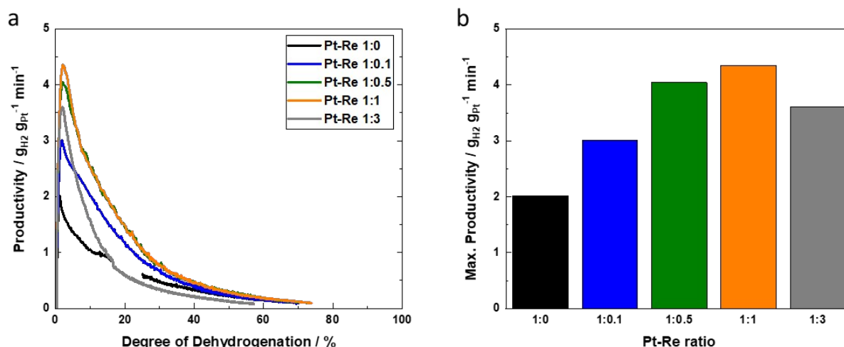
Figure 8: (a) Productivity and (b) maximum productivity at low conversions during dehydrogenation of H12-BT. Reaction conditions: 250 °C, 1 atm, 0.0001 mol Pt mol -1 LOHC , 31.01 g H12-BT , 0.30 wt.% Pt, 0-0.90 wt.% Re, 1320 min, 300 mL Ar min -1 . Calculations according to Equation (3) based on TCD analysis of released H 2 .
