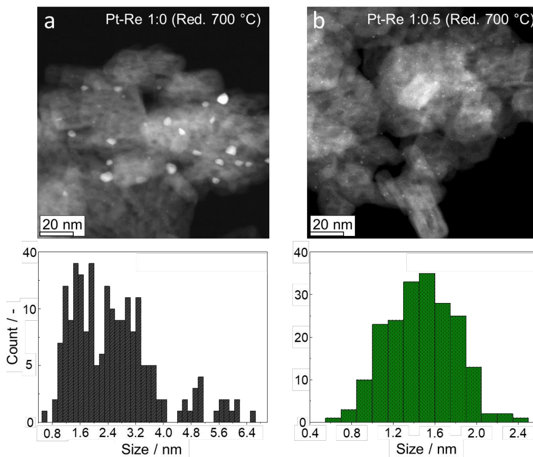
Figure 9: High-angle annular dark field scanning transmission electron micrographs of (a) a monometallic Pt-Re 1:0 and (b) a bimetallic Pt-Re 1:0.5 after reduction at 700 °C for 120 min with histograms of the size distribution.
