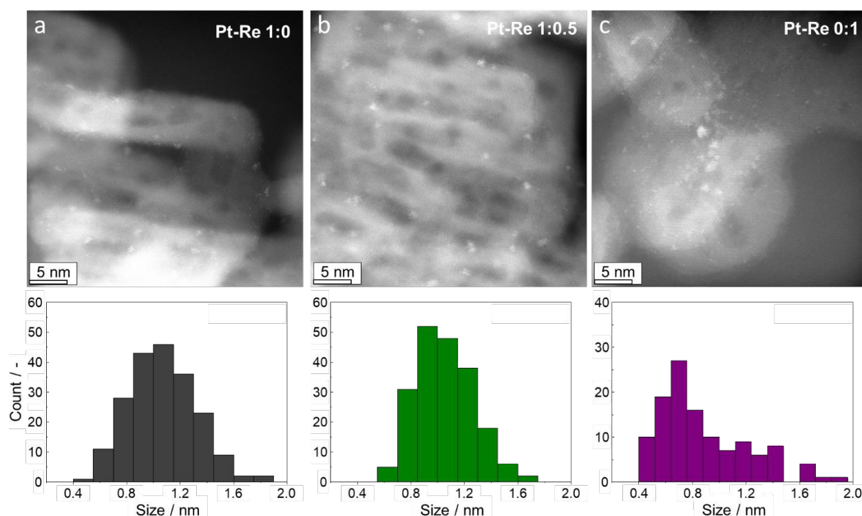
Figure 1: High-angle annular dark field scanning transmission electron micrographs of (a) the monometallic Pt-Re 1:0, (b) the bimetallic Pt-Re 1:0.5, and (c) the reference sample Pt-Re 0:1 with histograms of the size distribution. Note, that only clusters >0.4 nm were measured.
