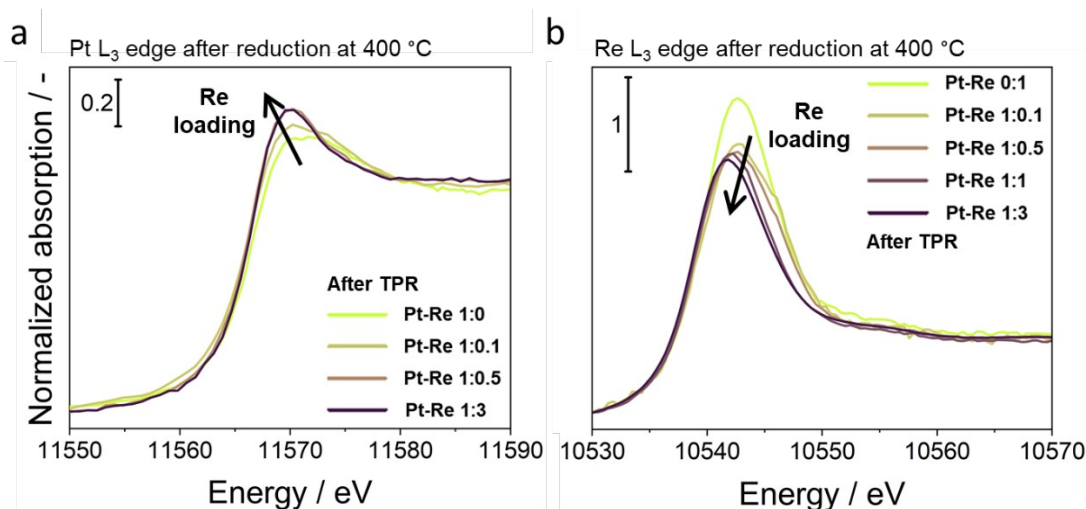
Figure 4: Comparison of in situ X-ray absorption spectra at (a) the Pt and (b) Re L_3 edge after reduction of the bimetallic Pt-Re catalysts with various ratios at 400 °C for 30 min with 10 °C min -1 in 11% H 2 /He. Spectra were acquired after cool-down to room temperature in 11% H 2 /He.
