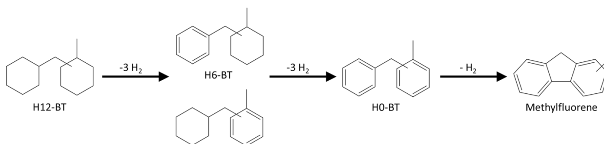
Figure 7: Reaction scheme of the dehydrogenation of perhydro benzyltoluene including undesired “deep” dehydrogenation via the formation of methylfluorene species.
