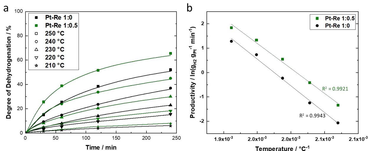
Figure 13: Degree of dehydrogenation during H_2 release from H12-BT at various temperatures using monometallic Pt-Re 1:0 and bimetallic Pt-Re 1:0.5 catalysts (a) together with an Arrhenius plot comparing the productivity at 5% DoDH (b). Reaction conditions: 210–250 ^{\circ}\text{C} , 1 atm, 0.0001 \text{ mol}_{Pt} \text{ mol}^{-1}_{LOHC} , 31.01 \text{ g}_{H12-BT} , 0.30 wt.% Pt, 0 or 0.15 wt.% Re, 240 min, 300 \text{ mL}_{Ar} \text{ min}^{-1} . Calculations for symbols according to Equation (5) are based on GC-FID analysis of liquid samples, while the solid lines are obtained according to Equation (2) based on TCD analysis of released H_2 .
