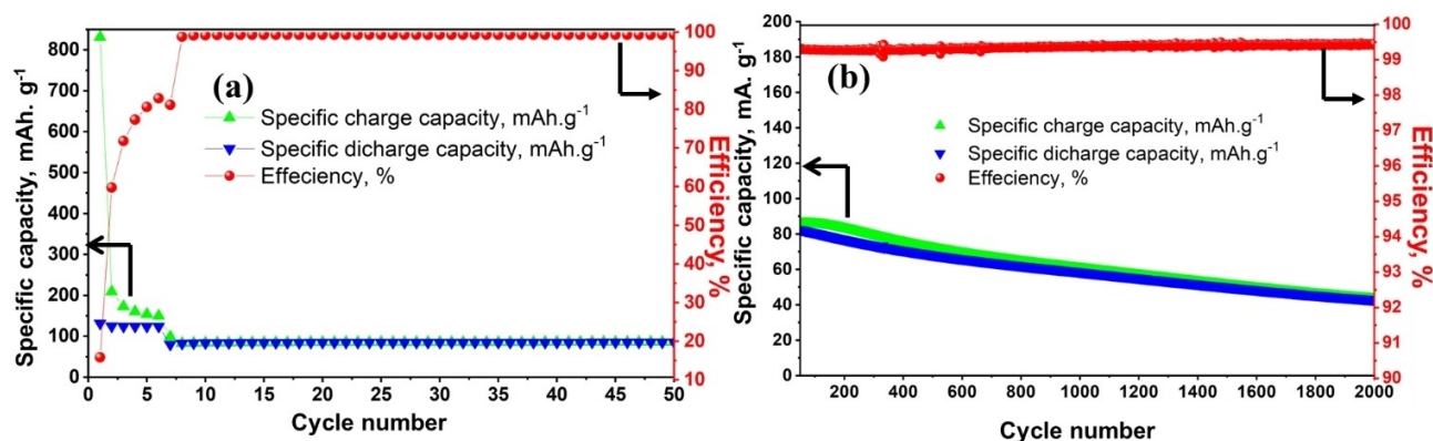
Figure 3. Cyclic performance of TDPP at 1 A g -1 a) 50 cycles in which the initial five cycles were performed at 0.1 A g -1 b) 2000 cycles.
