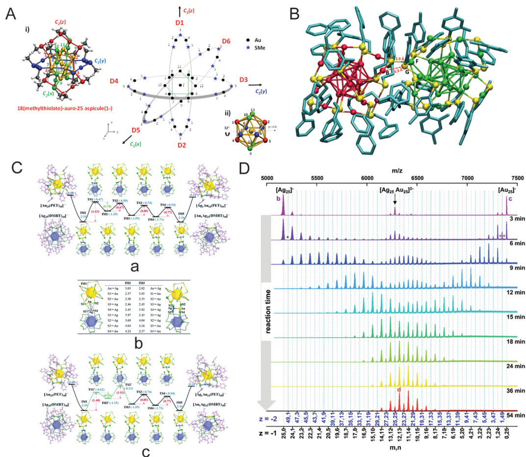
Fig. 11 (A) Borromean rings diagram of Au_{25}(SMe)_{18} , (B) DFT-optimization of the structure of [Ag_{25}Au_{25}(DMBT)_{18}(PET)_{18}]^{2-} adduct (with Ag_{25} on the left and Au_{25} on the right) as obtained from a force-field-based molecular docking simulation, (C) energy profiles of the metal exchange reaction between the [Au_{25}(PET)_{18}]^{-} and [Ag_{25}(DMBT)_{18}]^{-} nanoclusters; (a) path 1 initiated by Au-S PET bond breaking, (b) DFT optimized metal-metal and metal-S bond lengths (in Angstrom) (c) path 2 initiated by Ag-S DMBT bond breaking, and (D) time-dependent mass spectra of a 1 : 1 mixture of [Au_{25}(PET)_{18}]^{-} and [Ag_{25}(DMBT)_{18}]^{-} . Reproduced with permissions from ref. A–B, 166 C, 270 and D. 271 Copyright 2015 and 2021 American Chemical Society. Copyright 2016, The Royal Chemical Society.
