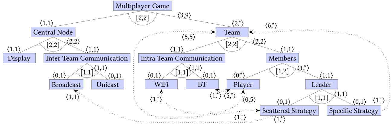
Figure 1: Cardinality-Based Feature Model of a Competitive Mobile Multi-Player Game
