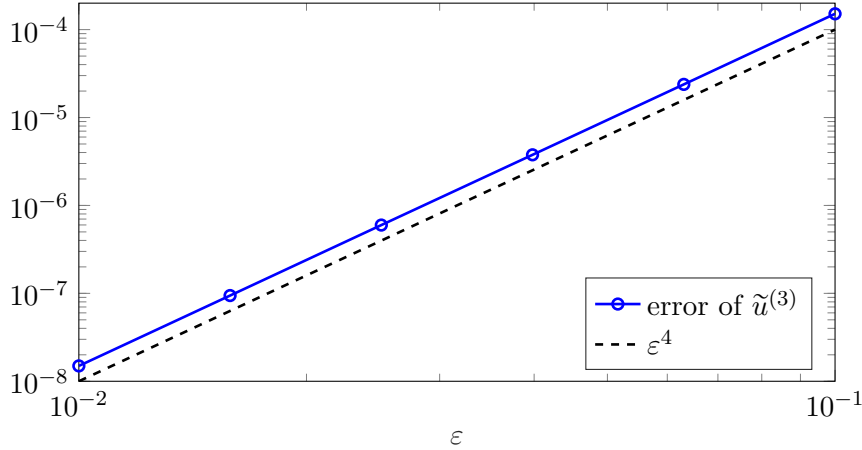
Figure 2: Accuracy of \tilde{u}^{(3)} for different values of \varepsilon . Parameters, data and discretizations are the same as in the numerical experiment described in Section 4.2.
