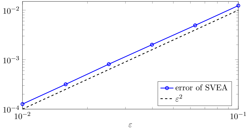
Figure 1: Accuracy of the SVEA for different values of \varepsilon . See text for details.
