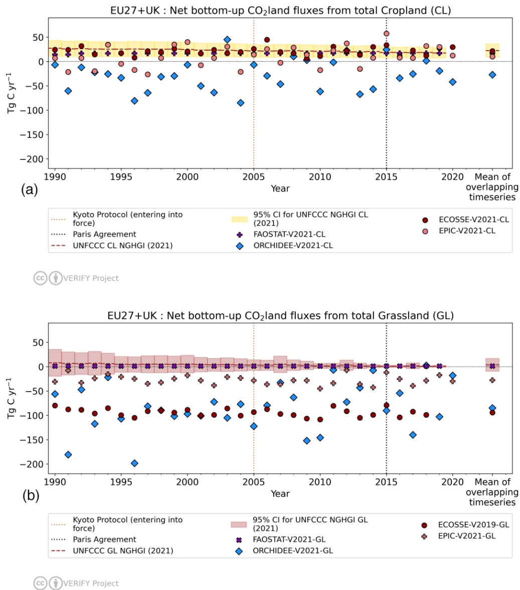
Figure 4. Net CO 2 land flux from total Cropland (a) and total Grassland (b) estimates for the EU27+UK. Total Cropland (CL) data come from the UNFCCC NGHGI (2021) submissions; ORCHIDEE, ECOSSE, and EPIC-IIASA process-based models; and the FAOSTAT inventory. Total Grassland (GL) data come from the same sources, with the caveat that ECOSSE has not been updated and is therefore identical to Petrescu et al. (2021). Values on the far right in both plots indicate the mean of 1990–2019. The relative error on the UNFCCC value represents the UNFCCC NGHGI (2021) MS-reported uncertainty with no gap filling (EU NIR, 2021). The fluxes follow the atmospheric convention, where negative values represent a sink, while positive values represent a source.
