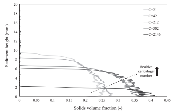
Fig. 4 Spatial distribution of solids volume fraction in a limestone sediment as a function of centrifugal acceleration. The measurement requires a two-step measuring procedure. First, suspension is centrifuged with the LUMiSizer analytical centrifuge at a speed. Subsequently, the sediment structure is investigated with X-Ray measurement with the LUMiReader X-Ray.
