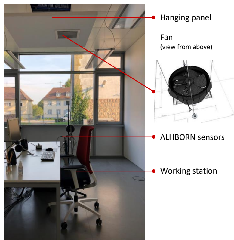
Figure 3. Setup of ceiling fan, sitting position, and sensors in the office room in the test chamber.
