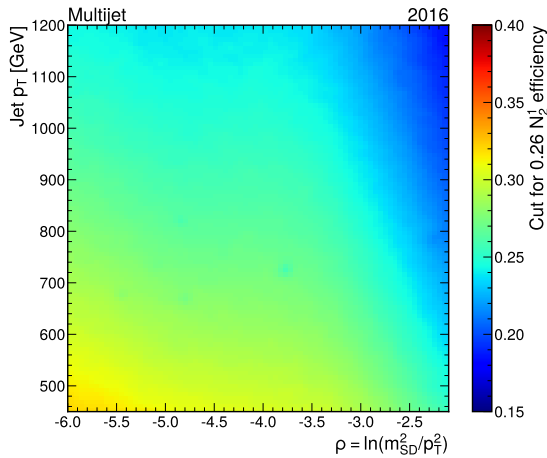
Figure 11.5: Transformation map of N_2^1 \rightarrow N_2^{1,DDT} , corresponding to a background efficiency of 26%, as a function of p_T and \rho . The z-axis correspond to X_\epsilon(p_T, \rho) in Eq. 11.5. The inflection in the distribution around \rho = -2 stems from the finite cone effect, and represents a natural limit to the mass of a QCD jet for a given p_T .
