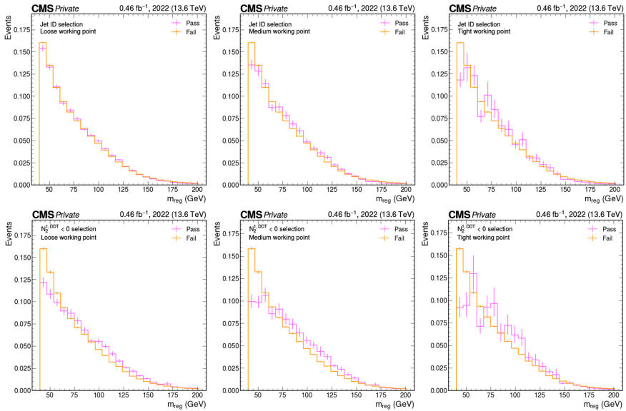
Figure A.1: Normalised event yield as a function of m_{reg} for collision data collected by the scouting stream in 2022. The upper and lower rows display the events before and after requiring N_2^{1,DDT} < 0 , respectively. The signal and control regions are shown in pink and orange. The left, middle and right columns display the partitioning into regions by the loose, medium and right DDB s WPs, respectively.
