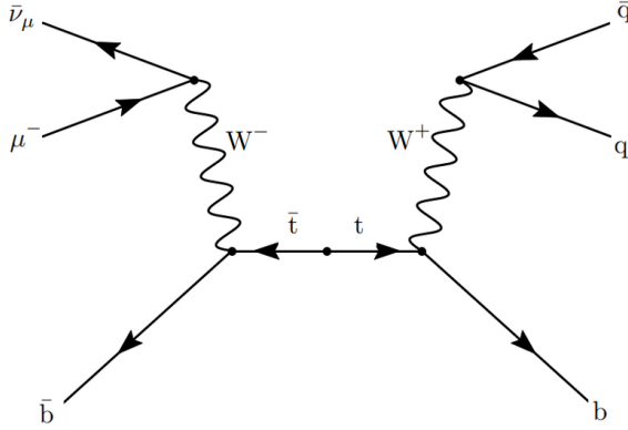
Figure 11.7: Feynman diagram of a single- \mu t\bar{t} event.
