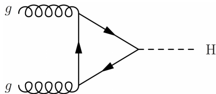
Figure 8.1: Feynman diagram of Higgs boson production through gluon-gluon fusion, where g denotes a gluon and H a Higgs boson.
