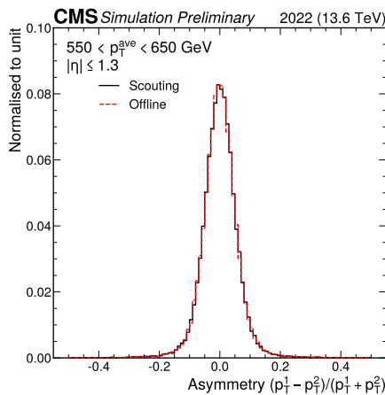
Figure 7.8: Comparison of asymmetry distributions of the scouting and offline reconstructions for simulated events with 550 < p_T^{\text{average}} < 650 and |\eta| < 1.3 . The histograms are normalised to unit. Author's contribution to Ref. [58].
