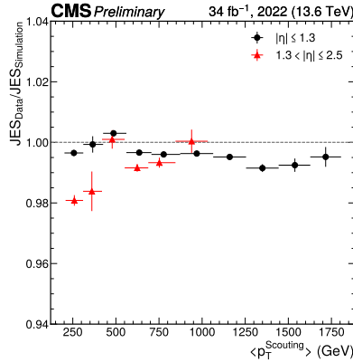
Figure 7.7: The ratio of the JES derived from collision data to the JES derived from simulation. The uncertainty is entirely statistical and is computed through error propagation of the numerator and denominator whose uncertainty is defined as the standard deviation of Eq. 7.15. Author’s contribution to Ref. [58].
