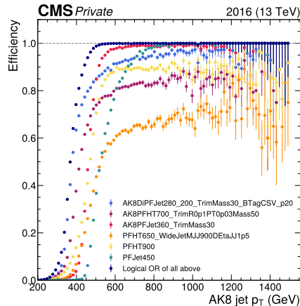
Figure 11.4: Trigger efficiency of the HLT triggers used to select events for collision data collected in 2016, as a function of AK8 jet p_T . A logical ‘OR’ of all the triggers is displayed in dark blue and reaches a plateau around 500 GeV. The uncertainties are entirely statistical and computed as Clopper-Pearson intervals.
