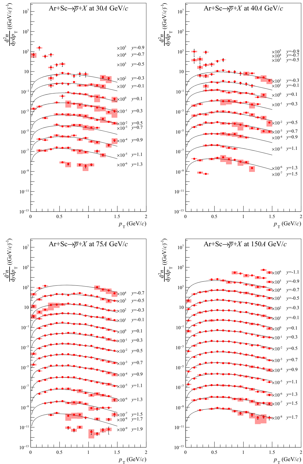
Fig. 58 Transverse momentum spectra in rapidity slices of \bar{p} produced in 10% most central Ar+Sc collisions at 30A to 150A GeV/c. For graphical presentations, the spectra are multiplied by factors given in the plots. Rapidity values given in the legends correspond to the middle of
