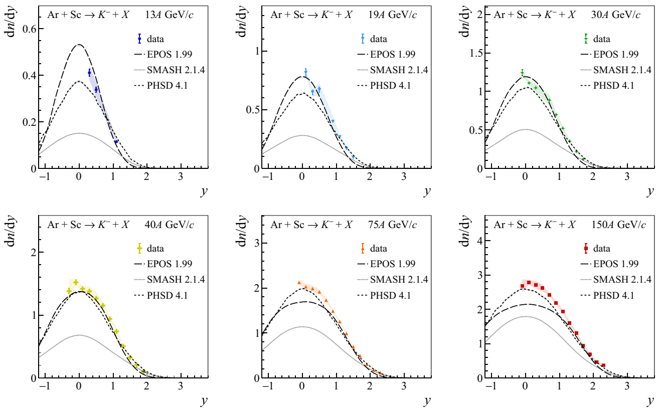
Fig. 44 Rapidity spectra of K^- mesons produced in 10% most central Ar+Sc interactions at 13A, 19A, 30A, 40A, 75A and 150A GeV/c in comparison with models: EPOS 1.99 [68], PHSD 4.1 [69, 70] and SMASH 2.1.4 [71, 72]
