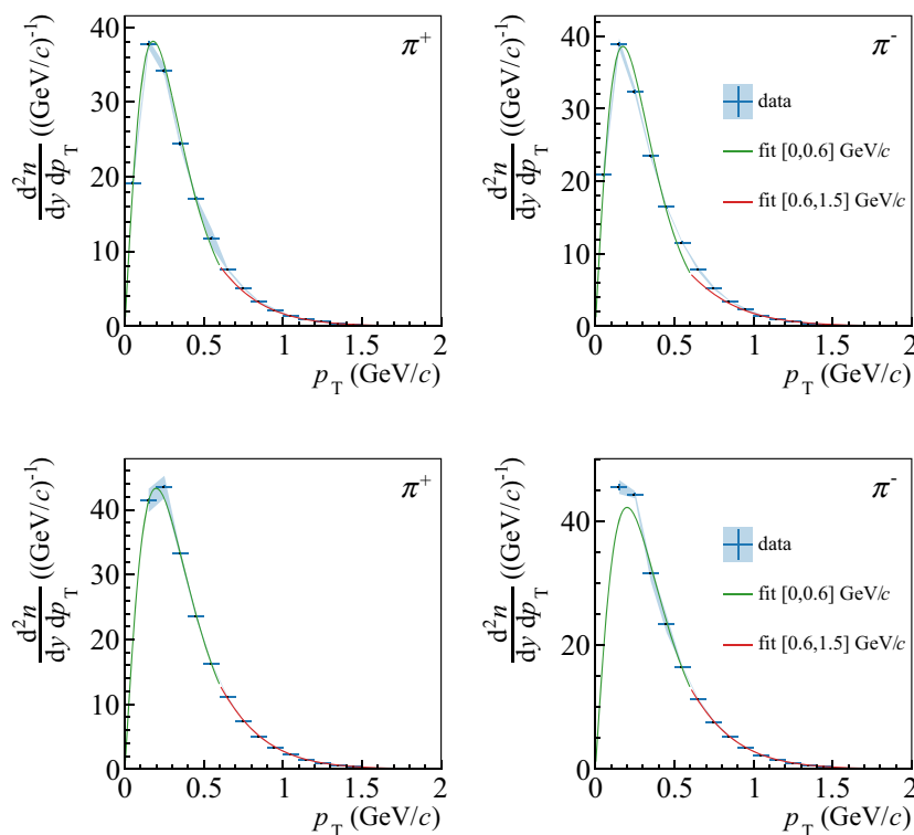
Fig. 19 Example fits to charged pion, \pi^+ (left) and \pi^- (right), transverse momentum spectra ( p_{\text{beam}} = 30A \text{ GeV}/c and 75A \text{ GeV}/c at 0.6 < y < 0.8 , top and bottom panels respectively). Exponential fits (Eq. 18) are performed in two regions separately: p_T \in [0.0, 0.6] and p_T \in [0.6, 1.5] \text{GeV}/c . The fitted functions are used to extrapolate the yields beyond p_T = 1.5 \text{ GeV}/c and interpolate the yields in case a gap
