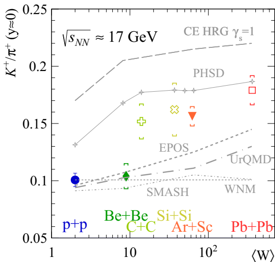
Fig. 52 System size dependence of the K^+/\pi^+ ratio (at y \approx 0 ) in central nucleus-nucleus and inelastic p+p interactions obtained at beam momenta of \approx 150A GeV/c ( \sqrt{s_{NN}} \approx 17 GeV) compared with dynamical (EPOS 1.99 [68], PHSD 4.1 [69, 70] and UrQMD [75, 76]) and statistical (HRG [77]) models. Additionally, WNM [25] prediction is shown as a horizontal dashed line
