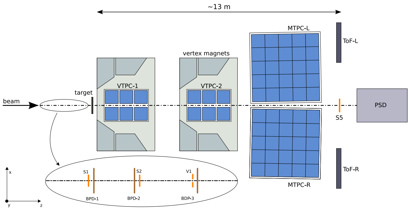
Fig. 1 The schematic layout of the NA61/SHINE experiment at the CERN SPS [18] showing the components used for the Ar+Sc energy scan. The beam instrumentation is sketched in the inset. The alignment of the chosen coordinate system as shown in the figure. The nominal
