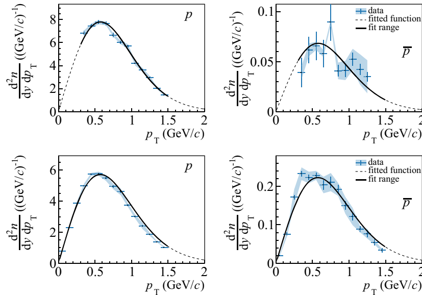
Fig. 28 Example fits to transverse momentum spectra of protons and anti-protons in 10% most central Ar+Sc collisions (top: p_{\text{beam}} = 30A GeV/c at -0.2 < y < 0.0 and bottom: p_{\text{beam}} = 150A GeV/c at 1.0 < y < 1.2 ). The fitted functions are used to extrapolate the yields beyond p_T = 1.5 GeV/c and interpolate the yields in case a gap in acceptance appears due to the different coverage of the PID methods.
