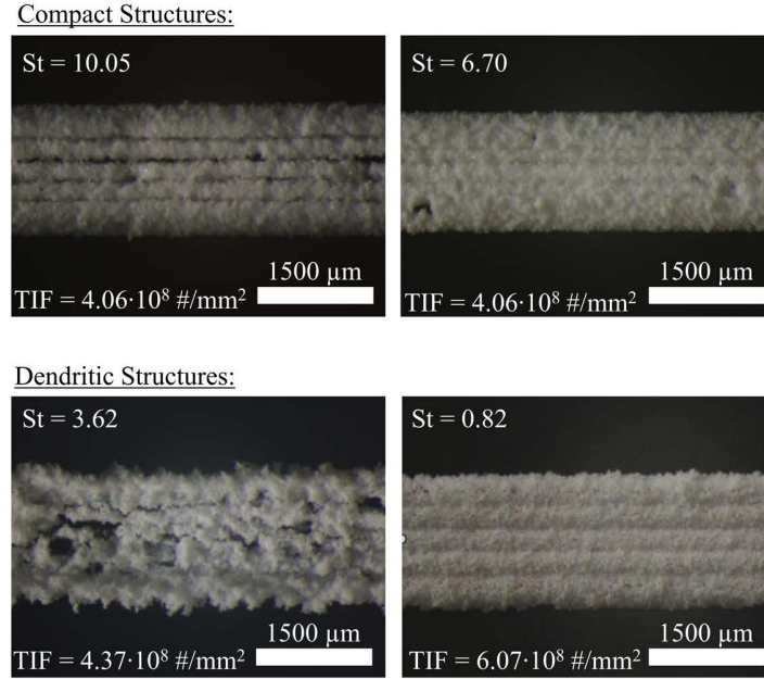
Figure 13: Morphology of the clogged particle structures on the fiber array as a function of the Stokes number.
