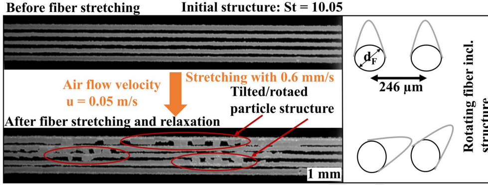
Figure 11: Left: Image section of the fiber array before stretching and after the 2nd stretching cycle for compact structures with a Stokes number of 10.05. Right: Schematic representation of the tilting of the particle structures into the fiber interspaces during stretching. No reversal of the tilted particle structure after relaxation of the fiber.
