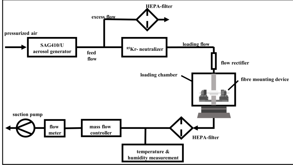
Figure 4: Schematic setup to produce an aerosol containing glass spheres and the deposition on an fiber array that is clamped at the fiber mounting device [5].
