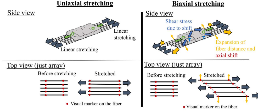
Figure 17: Schematic on the differences between uniaxial and biaxial stretching in side and top view. The stretching and displacement of the fibers are indicated by visual markers in the case of biaxial elongation.
