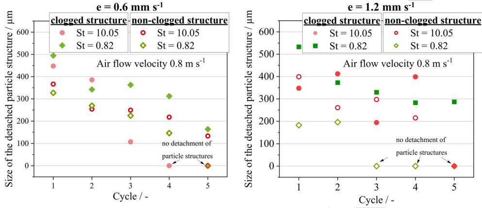
Figure 16: Mean size of detached agglomerates from the fiber array as a function of each single stretching cycles for a compact and a dendritic initial structure. The stretching velocity is varied from 0.6 \text{ mm/s} to 1.2 \text{ mm/s} . Size values of 0 indicate "no detachment".
