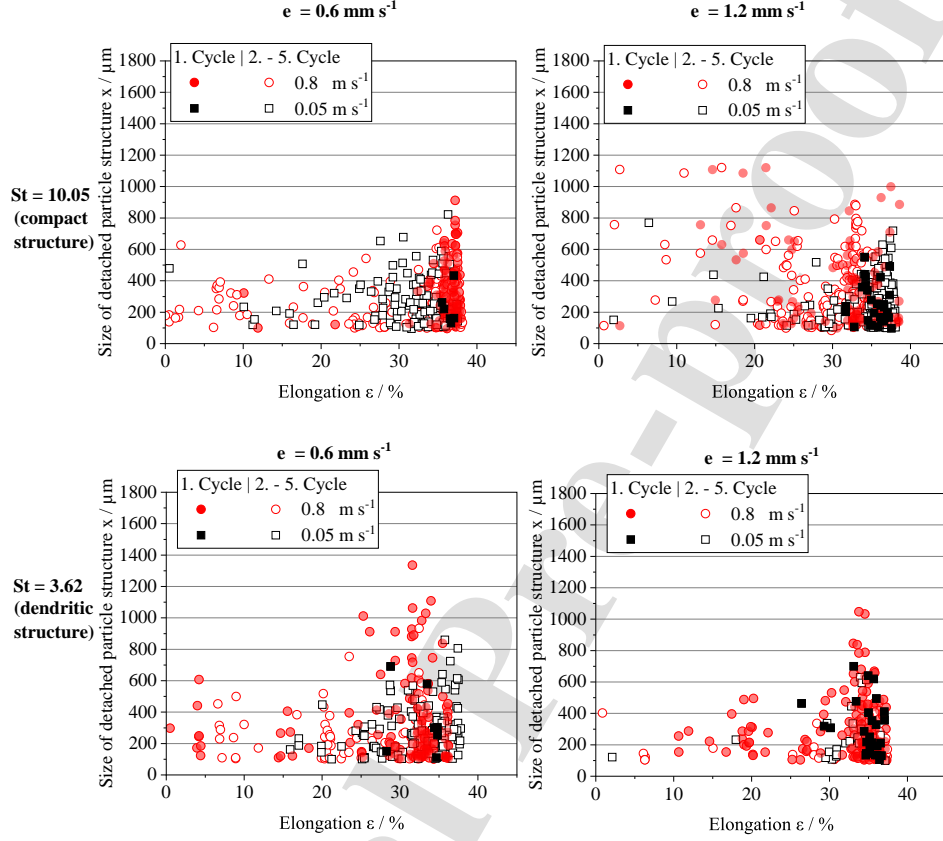
Figure 9: Size of the detached particle structures as a function of the structural morphology (TOP: St = 10.05 ; BOTTOM: St = 3.62 ; Left: 0.6 \text{ mm s}^{-1} ; Right: 1.2 \text{ mm s}^{-1} ), as well as the elongation and flow velocity.
