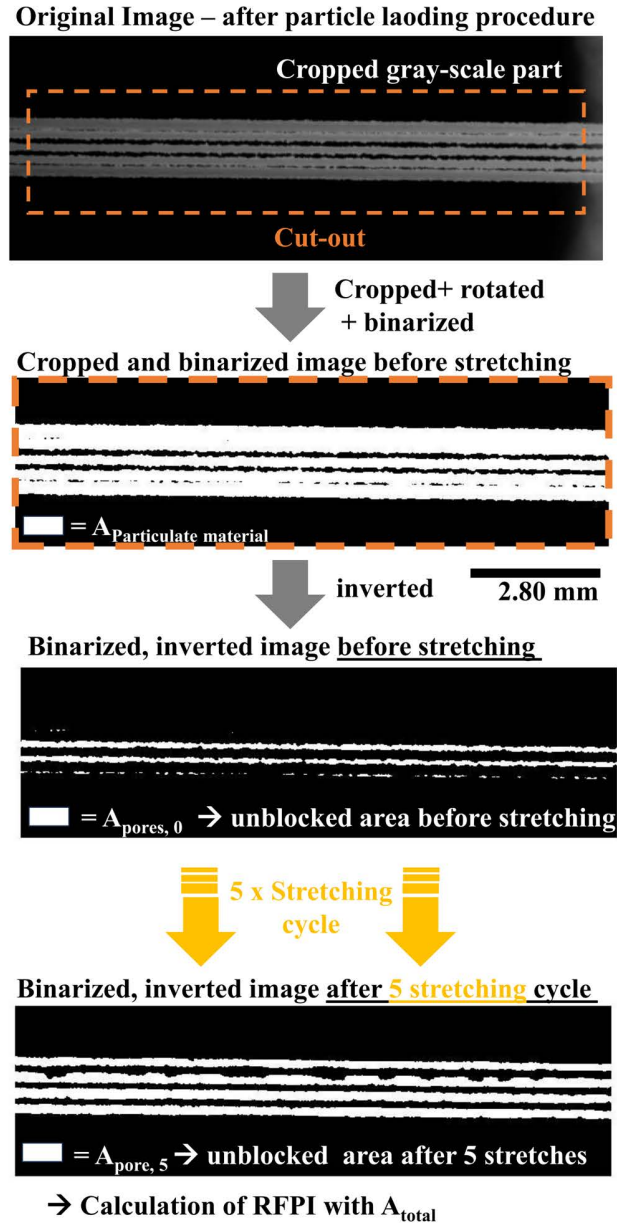
Figure 6: Schematic procedure for determining the proportion of unblocked area in the fiber interspaces of the array.
