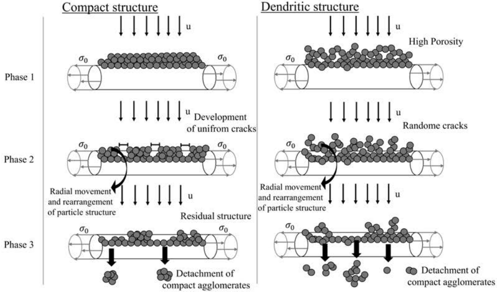
Figure 8: Schematic of the three phases of detachment. Left: compact structures, Right: dendritic structures. Crack building, radial rearrangement of particle structures and detachment are visible.
