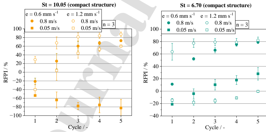
Figure 10: RFPI of the stretching experiments with a compact particle structure on the fiber array.
