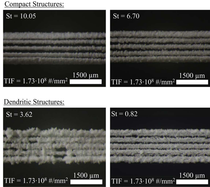
Figure 7: Morphology of the non-clogged particle structures on the fiber array as a function of the Stokes number.
