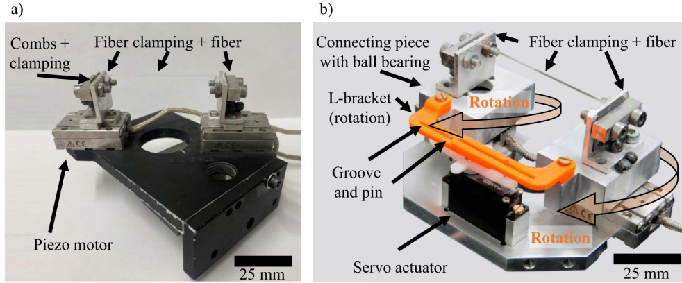
Figure 2: a) Clamping device for just stretching the fiber array b) Clamping device for simultaneous stretching and changing the fiber distance by rotating the clamping combs.
