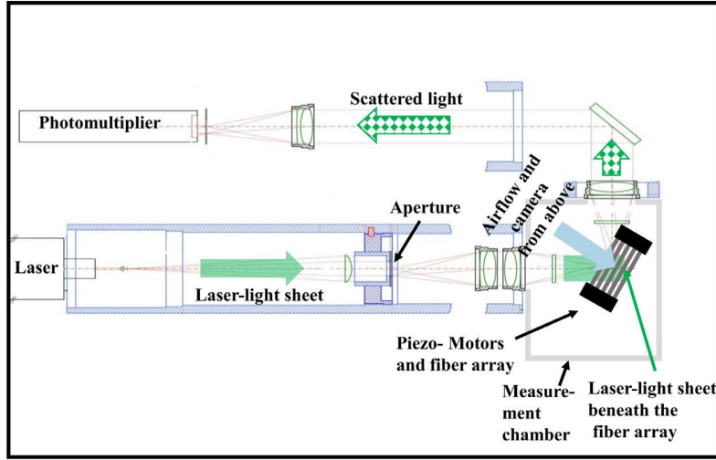
Figure 5: Schematic diagram of the laser thin film measurement system. An expanded laser beam (thin sheet) passes beneath the fiber array. The scattered light within the measurement area is focused onto a photomultiplier and converted into electrical pulses.
