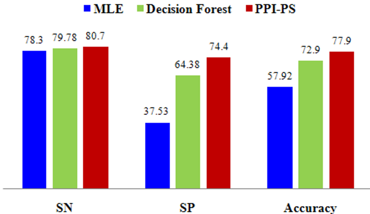
Figure 2 Comparing PPI-PS performance with MLE and Domain-based random forest of decision trees methods.
