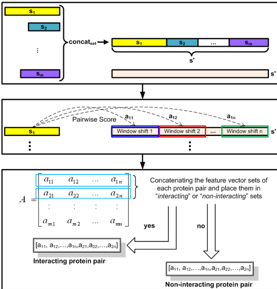
Figure 4 Overview of the feature extraction step.
