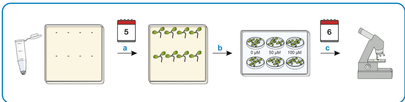
Figure 6. Workflow to analyze inducible target cell ablation in the root apical meristem (RAM)
