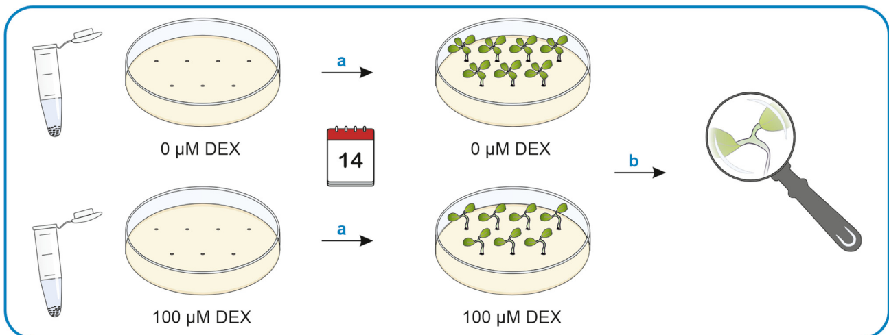
Figure 4. Workflow to analyze inducible target cell ablation in seedlings
