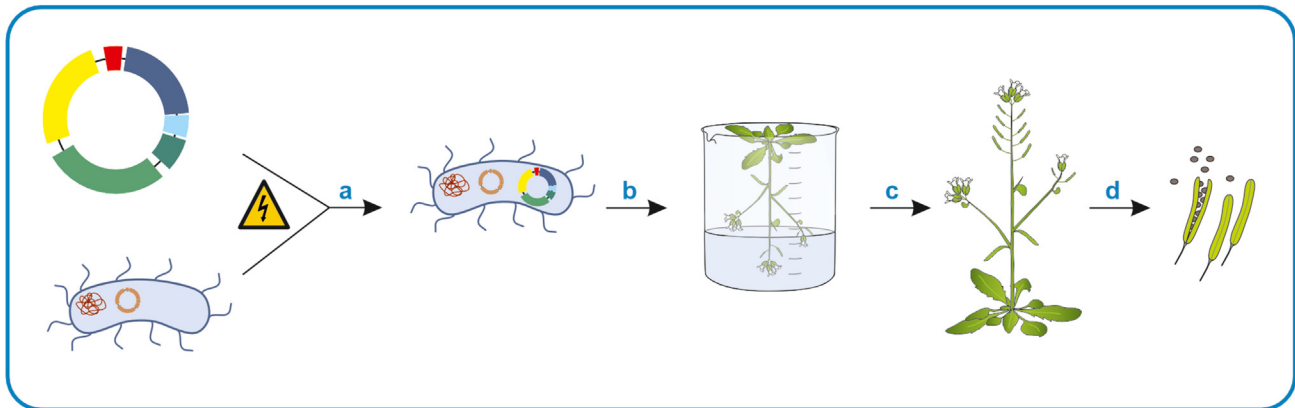
Figure 1. Workflow for generating constitutive, uninducible CRISPR-Kill lines
