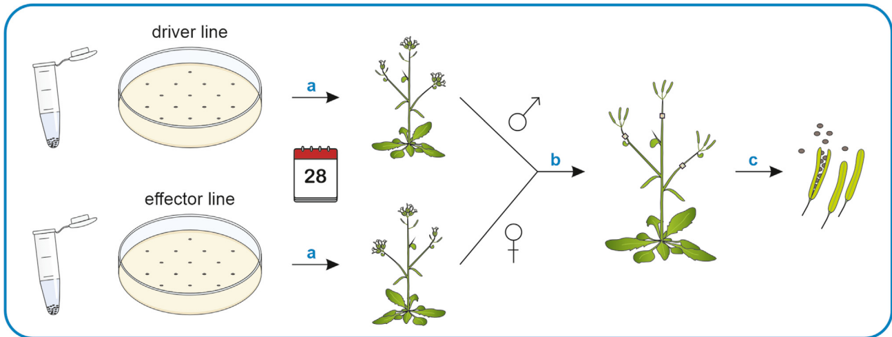
Figure 2. Workflow for generating DEX-inducible tissue-specific CRISPR-Kill expression lines
