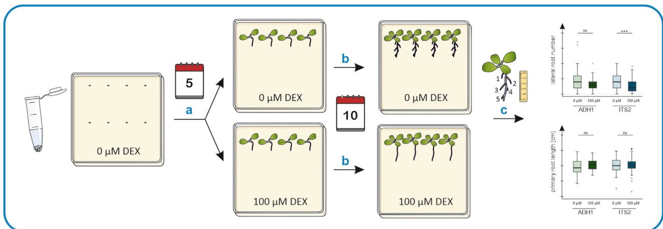
Figure 5. Workflow to analyze inducible target cell ablation in the root
