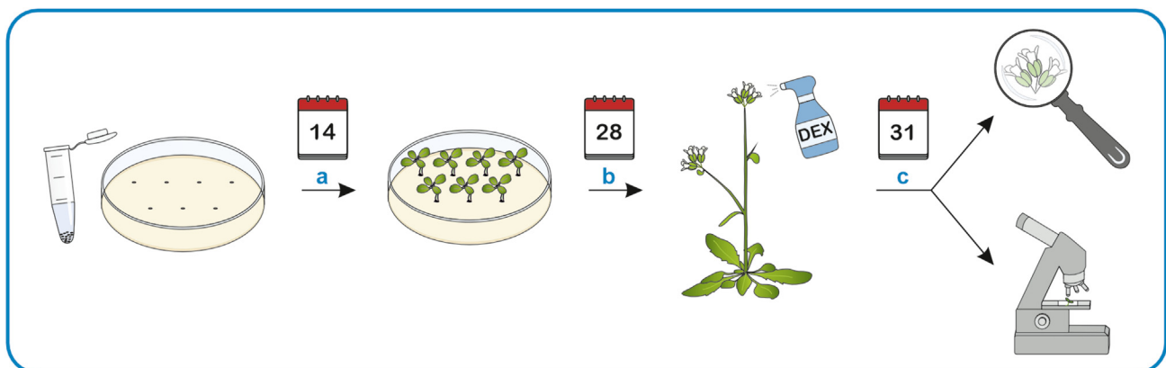
Figure 7. Workflow to analyze inducible target cell ablation in the shoot apical meristem (SAM)
