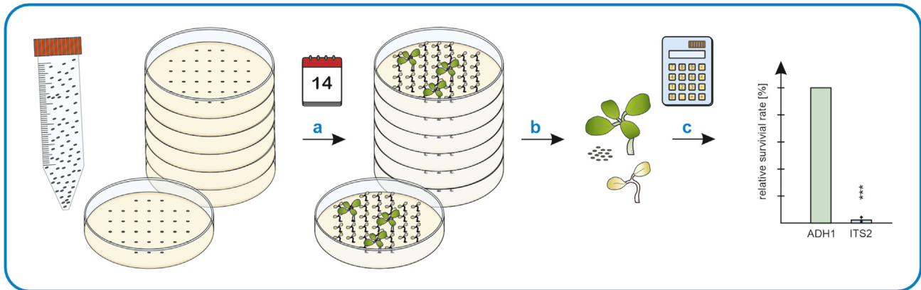
Figure 3. Workflow to analyze constitutive target cell ablation macroscopically
