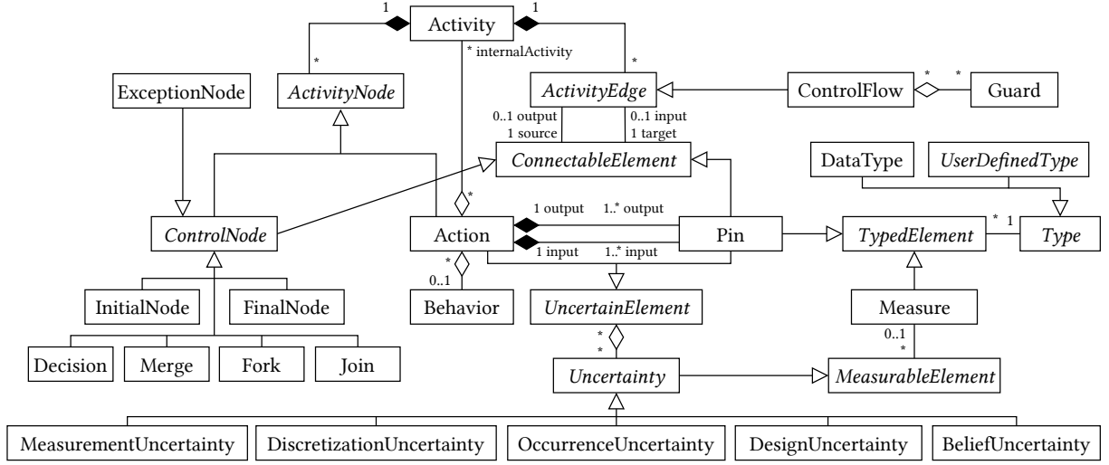
Figure 4: Uncertainty Flow Diagram (UFD) metamodel showing the relation of activities, flows, and different uncertainty types.
