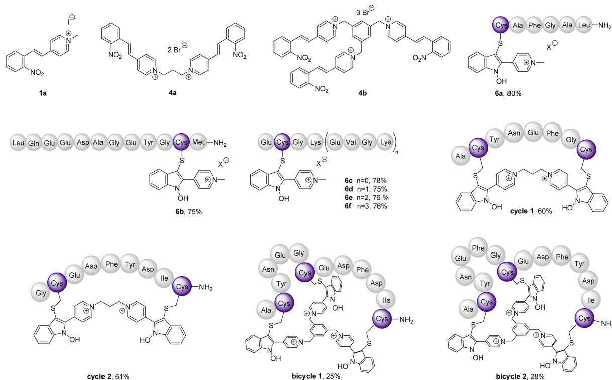
Fig. 3 Selective modification of one, two or three sulfhydryl groups in peptides with mono-, bi- and trifunctional 4-(2-nitro-5-styryl)pyridinium linkers. Conditions for the coupling reactions: peptides with a single cysteine residue: 2.0 mM 1a , 1.5 equiv. peptide 5a–5f , 100 mM \text{NH}_4\text{HCO}_3 buffer (pH 8.0), 37 °C, 0.5–2 h; peptides with two cysteine residues: 0.50 mM 4a , 1.0 equiv. peptide 5g , 5h , 100 mM \text{NH}_4\text{HCO}_3 buffer (pH 8.0), rt, 1 hour; peptides with three cysteine residues: 0.20 mM 4b , 1.0 equiv. peptide 5i , 5j , 100 mM \text{NH}_4\text{HCO}_3 buffer (pH 8.0), 0 °C \rightarrow rt, 1 hour. Isolated yields; products purified by prep. HPLC.
