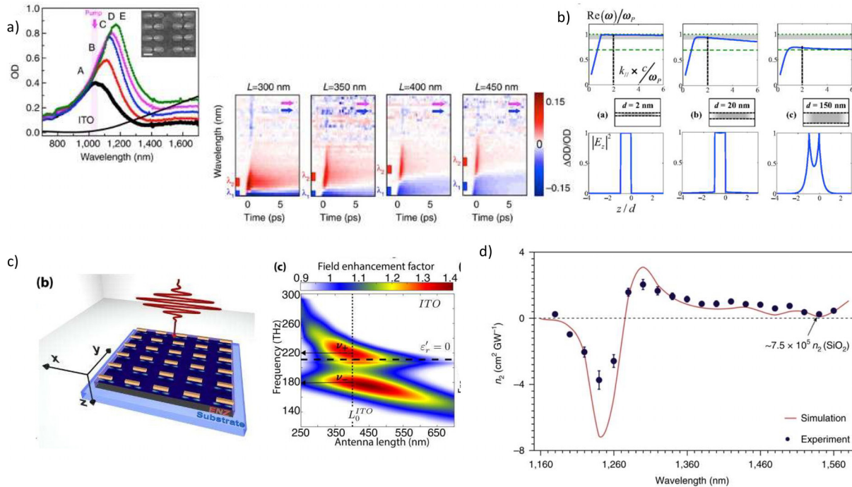
FIG. 37. Experimental demonstrations of plasmonic metasurfaces enhancing the nonlinear response of TCOs. a) Plasmonic dimers on ITO show a large, fast (sub-picosecond) modulation of optical density when exciting antenna resonances, suggesting a strong, fast Kerr-type nonlinearity. 1018 (b) A sufficiently thin, bare layer of ENZ material will support a Berreman (LR-SPP) mode with high field enhancement, but cannot easily couple to light in free space. 189 (c) Nanoantennas with resonances in the ENZ region of a thin TCO layer exhibit mode splitting from strong coupling between the metasurface and the LR-SPP mode. 1016 (d) When a metasurface enables optical pumping of this LR-SPP mode, it not only shows an enhanced nonlinear response but can also extend this nonlinear enhancement well beyond the narrow spectral range where \epsilon is near zero. 184 All images are reprinted (adapted) with permission from the respective Journal and copyright remains with the original publisher.
