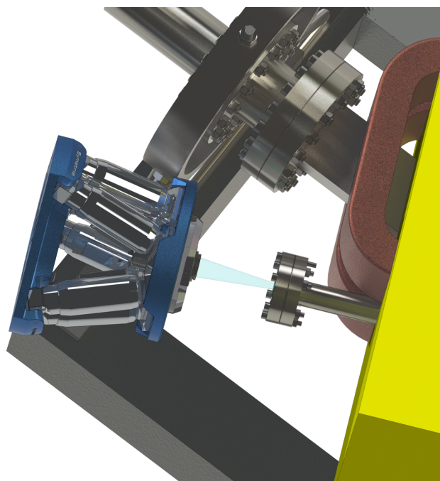
Figure 2: Six degree of freedom hexapod platform to align the fiber collimator to the synchrotron light beam coming out of one dipole magnet (Illustration shows hexapod as far away from the window as possible).
