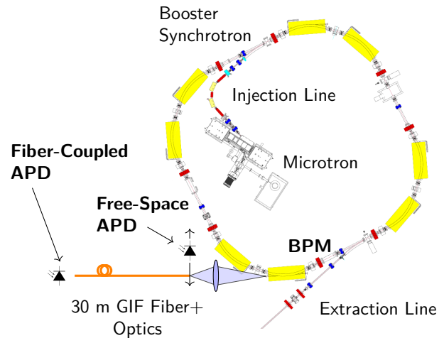
Figure 1: Booster synchrotron of KARA with added diagnostic elements; used detectors highlighted in bold.
