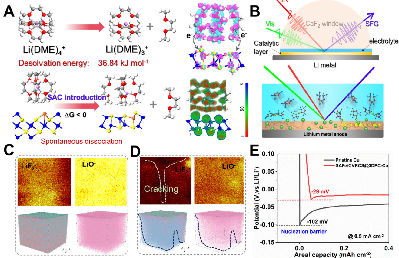
Fig. 3 (A) SAC accelerates \text{Li}(\text{DME})_n^+ desolvation. (B) Characterization of SFG in monitoring interfacial desolvation. TOF-SIMS of (C) SAFe/CVRCS@3DPC-Li and (D) original Li. (E) Nucleation overpotential. Reproduced with permission. 50 Copyright 2023, Wiley-VCH.
