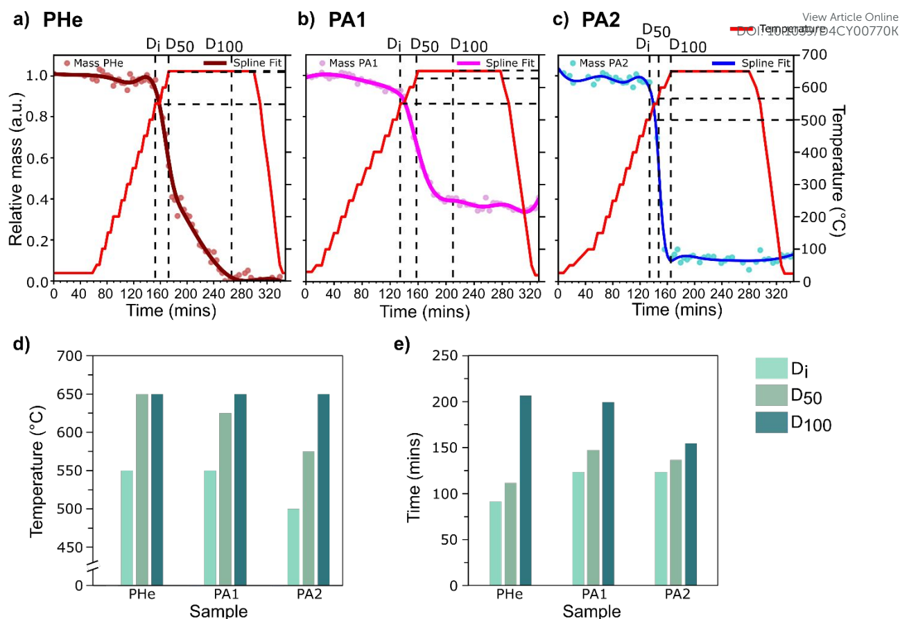
Figure 3: Relative change in mass of samples a) PHe, b) PA1, and c) PA2 over time, including temperature program during step-wise heating and cooling. The extent of catalyst restructuring is described using three different events, D_i , D_{50} , and D_{100} , and their corresponding d) temperature and e) treatment time for each sample. Time values were offset to account for the different absolute time points of the first heating ramps.
