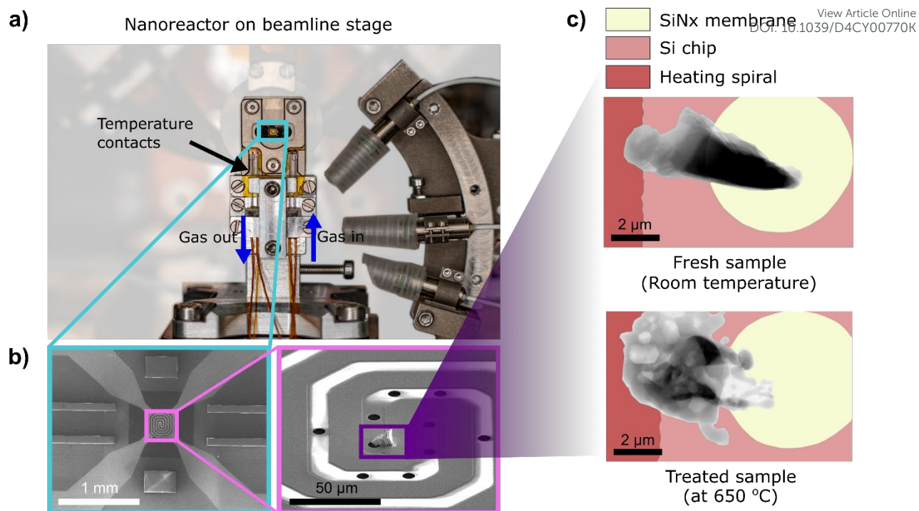
Figure 1: In situ nanoreactor a) implemented for use at synchrotron radiation sources, showing b) heating spiral (left) and zoomed-in view of the sample mounting region (right). c) Ptychographic projections (grayscale) of a fresh sample (top) mounted on a MEMS-based TEM chip, and a treated sample (bottom) illustrate changes in Ag catalyst morphology after exposure to elevated temperatures under different gas environments at atmospheric pressure in the nanoreactor.
