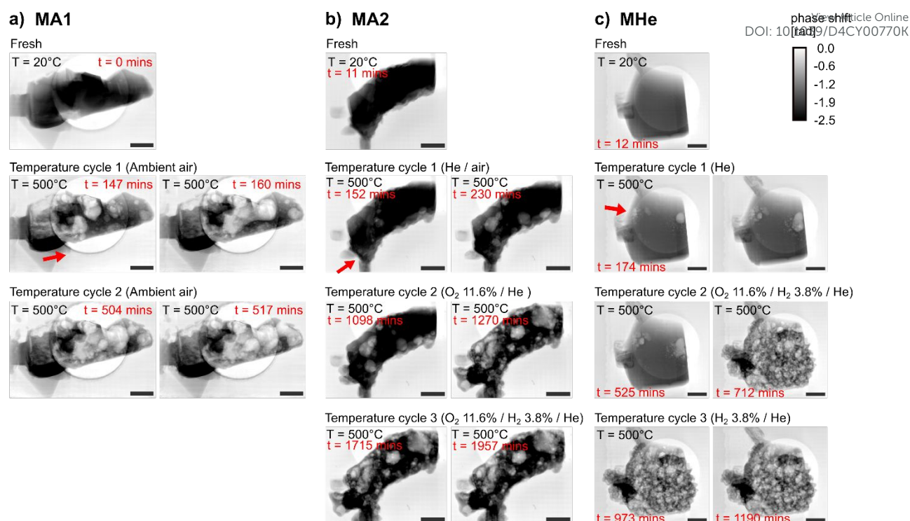
Figure 4: In situ X-ray ptychography projections of samples a) MA1, b) MA2, and c) MHe. The top row for each sample shows the fresh sample. The subsequent rows for each sample exhibit morphological changes at the start and end of each constant temperature condition of 500 °C, under their respective environments. The red arrows indicate bubble formation and the direction of bubble propagation. All scale bars = 2 \mu\text{m} .
