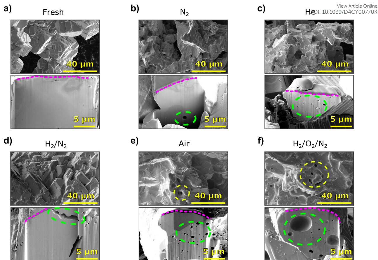
Figure 6: SEM image (top) and FIB-milled cross-sectioned SEM image (bottom) of Ag catalysts, a) fresh, and after 48 h of heat treatment under different gas environments: b) N 2 , c) He, d) H 2 /N 2 = 2/98 vol%, e) synthetic air and f) H 2 /O 2 /N 2 = 2/6/92 vol%. The Pt protection layer was deposited on the top surface before FIB milling (pink dashed line). The pores on the catalyst surface (yellow circles) and the cavities inside the catalyst exposed after FIB-milling (green circles) have been indicated.
