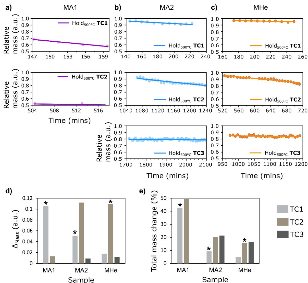
Figure 5: Relative change in mass in the selected ROIs plotted as a function of time to study the catalyst behavior at a constant temperature of 500 °C for three samples – a) MA1, b) MA2, and c) MHe. d) Bar chart showing change in mass ( ESI, Table S4 ) during each temperature cycle (denoted as TC) for all three samples. e) The corresponding percentage change in mass with respect to the initial mass, showing estimated percentage decrease in the observed ROI after each period of holding at a constant temperature. (* denotes the cycle with the first exposure of sample to O 2 ).
