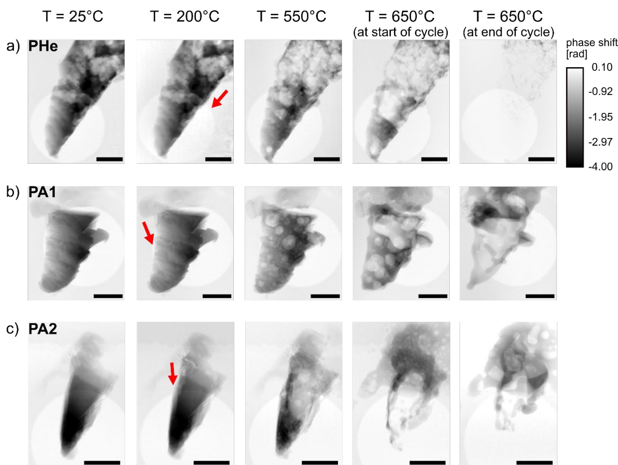
Figure 2: In situ X-ray ptychography projections of a) PHe, b) PA1, and c) PA2 as a function of applied temperature for T = 25, 200, 550, and 650 °C (showing start and end of the constant temperature cycle) under their respective gas environment. The
