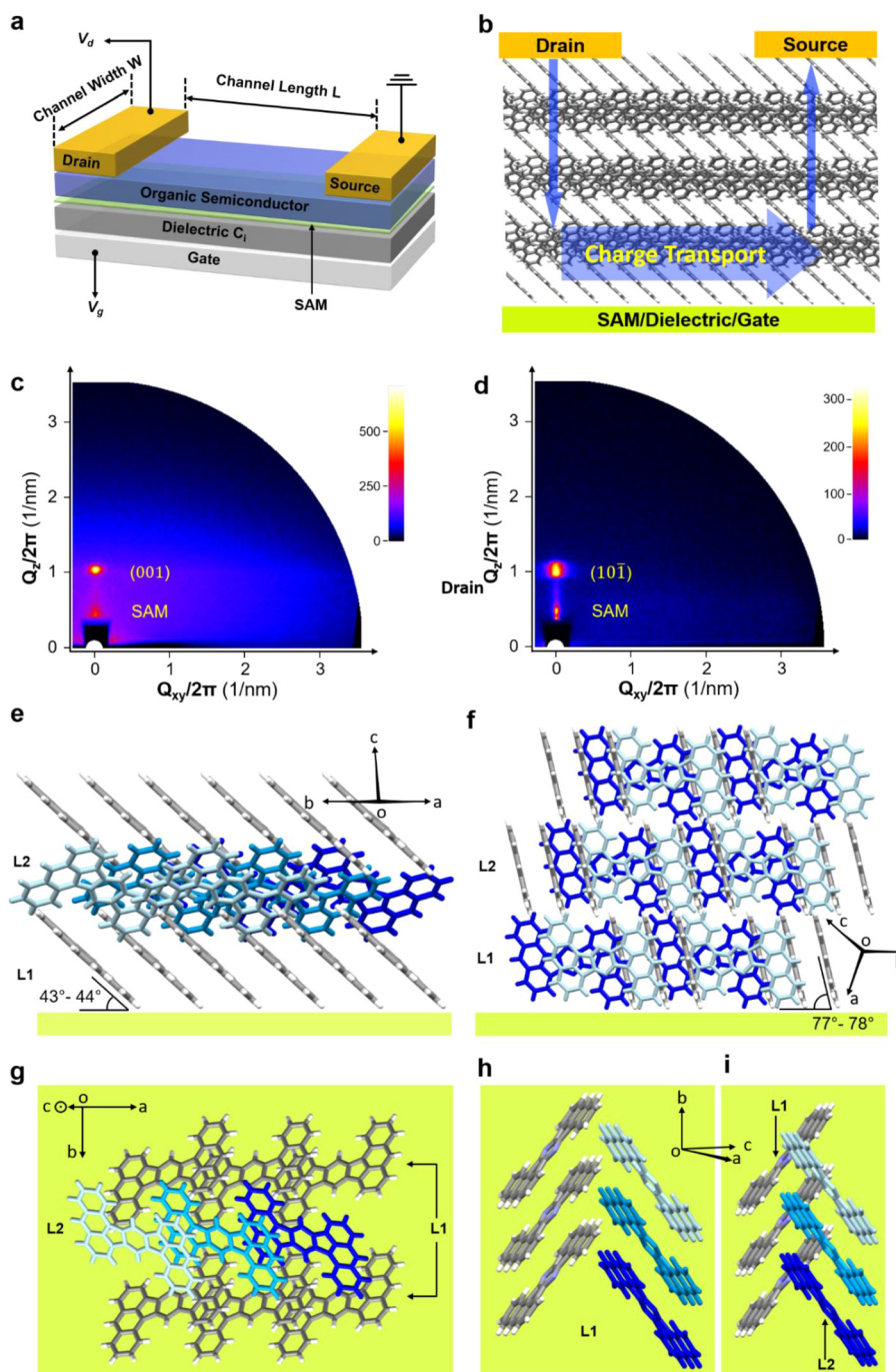
Fig. 7 Molecular orientation of DBAF and DBAF-N 2 at the organic/SAM/inorganic interface of the OTFT devices. (a) The OTFT device used in this work has a bottom-gate-top-contact structure. (b) Illustration of charge transport taking place in a working device of DBAF. (c) and (d) are typical GIWAXS data for the DBAF- and DBAF-N 2 -based devices, respectively. (e) Side view and (g) top view of the orientation of DBAF molecules. (f) Side view and (h and i) top views of the orientation of DBAF-N 2 molecules. (h) shows the first layer (L1) at the SAM/inorganic substrate (bright green). (g) and (i) show the first two layers, in which molecules colored in grey come from the first layer (L1) and molecules in various blue colors are from the second layer (L2).
