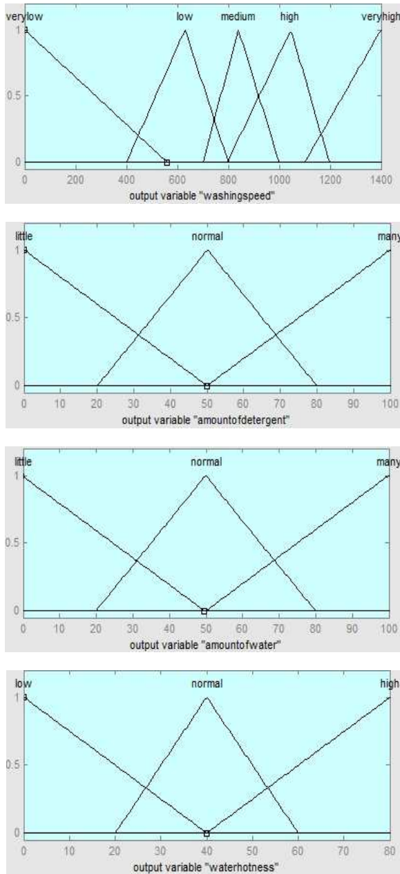
Figure 6. Fuzzy logic output membership functions
