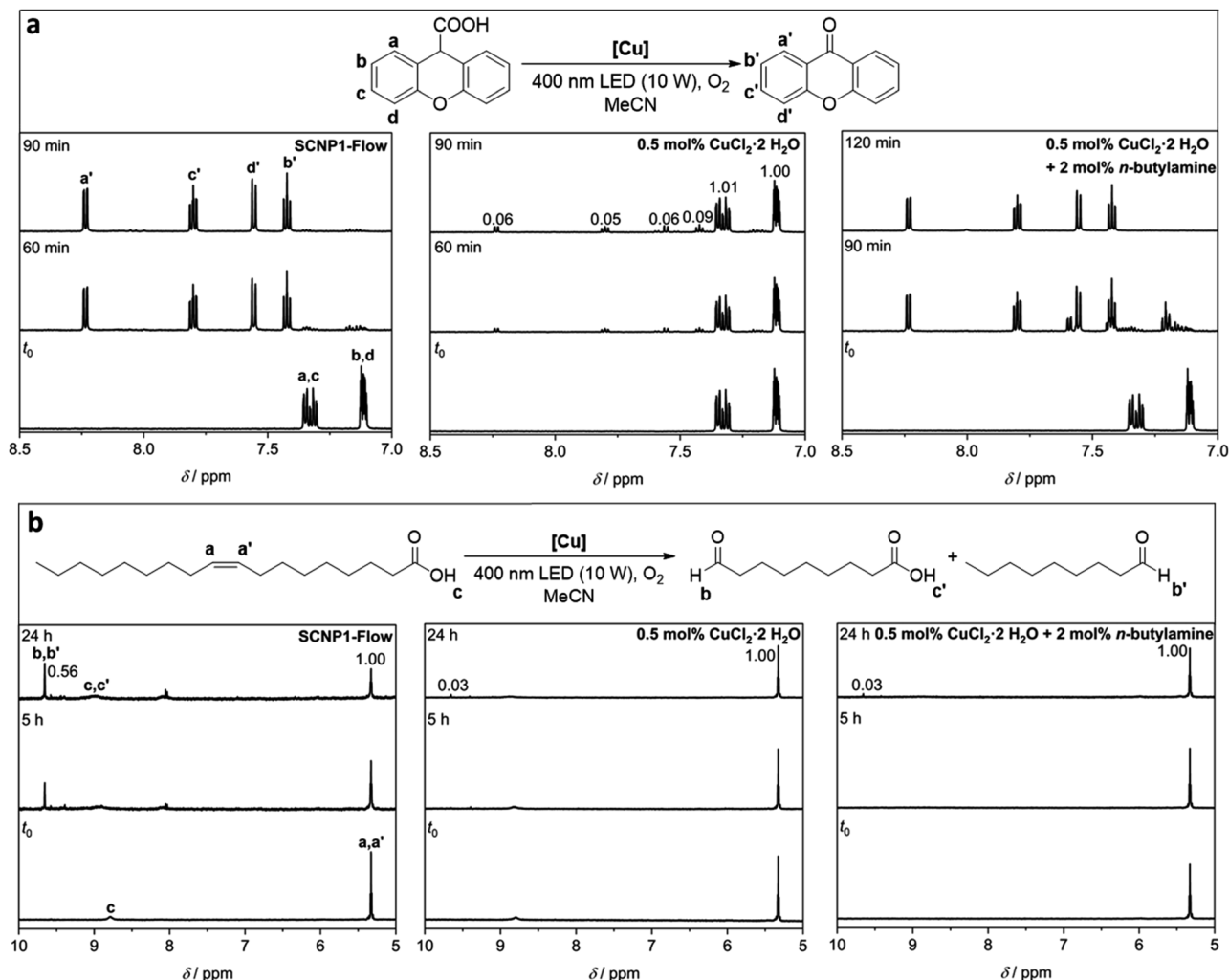
Fig. 4 Reaction schemes and 1 H NMR spectra (600 MHz, CD 3 CN, 298 K) of (a) the photocatalytic decarboxylation and oxygenation of xanthen-9-carboxylic acid and (b) the oxidative cleavage of oleic acid employing SCNP1-Flow (left), CuCl 2 ·2H 2 O (centre) or CuCl 2 ·2H 2 O in the presence of n -butylamine (right) as the catalyst. Resonance labels refer to the respective schemes above the spectra. Numbers on resonances denote integral values.
