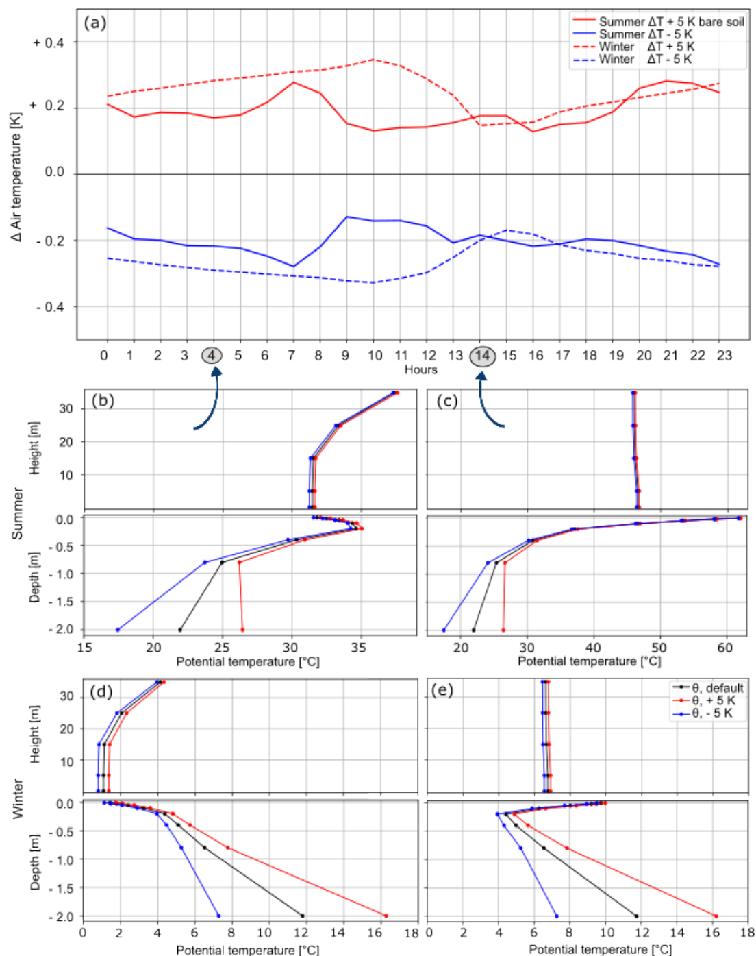
Figure 5. Potential air temperature modifications in 5 m height over a bare soil under cyclic boundary conditions for the whole third simulated day for winter and summer. Additionally, at 04:00 and 14:00 the potential soil- and the potential air temperature profile until a height of 35 m for the default scenario, +5 K, and -5 K deep soil temperature (-2 m) is shown.
