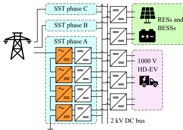
FIGURE 11: MW charger proposed in [149], [151].
