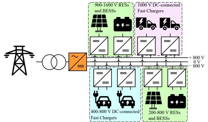
FIGURE 10: Example of DC-connected fast charging system in a bipolar architecture with a \pm 800 V DC bus. The idea of a total 1600 V DC bus was inspired by [48].
