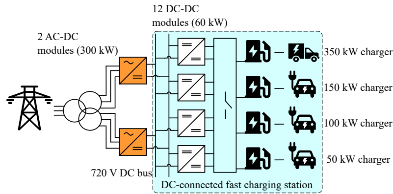
FIGURE 8: Power architecture of Enercon E-charger 600 [36], [37].
