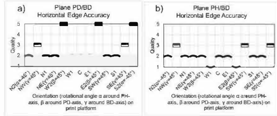
Fig. 4 Geometrical accuracy of the top horizontal edges of the test specimens viewed from the PD/BD (a) and PH/BD (b) side and rotated in different directions according to the given rotational angle (Quality criteria 1=concave, 2=convex, 3=below ideal shape, 4=exceeding ideal shape, 5=ideal shape)
