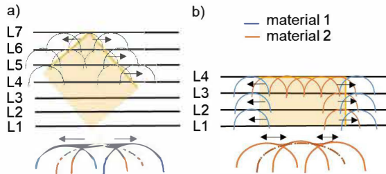
Fig. 5 Potential droplet coalescence scenario in this printing process
