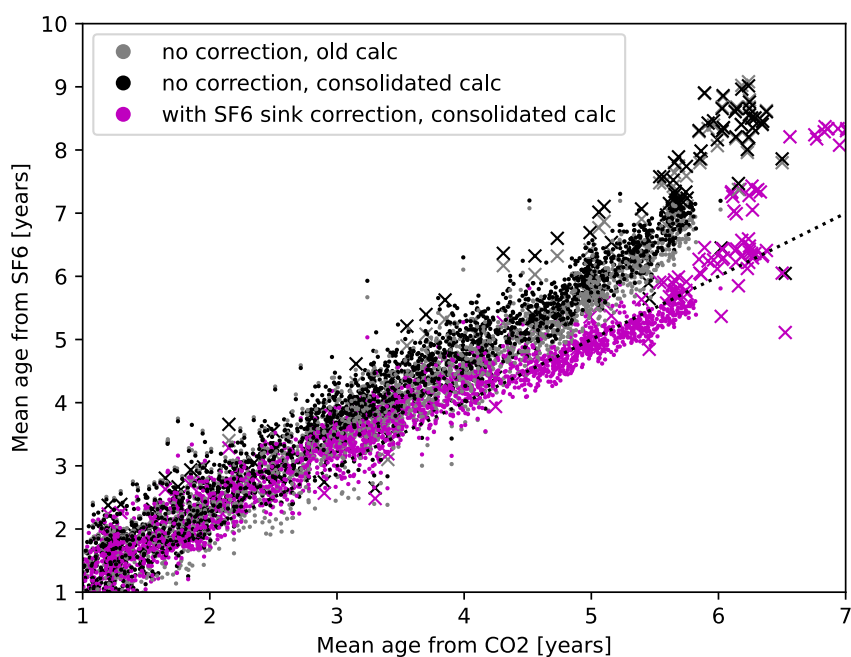
Figure 7. Mean age from aircraft data (dots) and balloon profiles (crosses) from concurrent observations of SF 6 and CO 2 for mean ages with the originally published calculation (gray), with the consolidated method for SF 6 (black), and in addition with the SF 6 sink correction applied (magenta).
