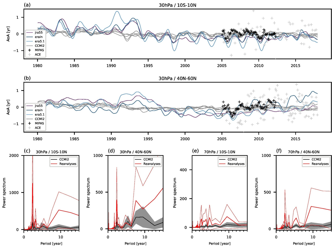
Figure 12. Mean age of air variability in reanalyses and climate models. (a) Deseasonalized anomaly of mean age in the tropics ( 10^{\circ}\text{S} – 10^{\circ}\text{N} ) at 30 hPa from CCM12 climate models (gray), reanalyses (colored), MIPAS (black crosses), and Atmospheric Chemistry Experiment Fourier Transform Spectrometer (gray crosses) satellite data. Panel (b) same, but in middle latitudes ( 40^{\circ}\text{N} – 60^{\circ}\text{N} ). (c–f) Power spectrum of mean age variability at 30 and 70 hPa, in the tropics ( 10^{\circ}\text{S} – 10^{\circ}\text{N} ) and in middle latitudes ( 40^{\circ}\text{N} – 60^{\circ}\text{N} ) for CCM12 (multi-model mean in black, 1 - \sigma range as gray shading) and reanalyses (multi-reanalysis mean as thick red, 1 - \sigma range as thin dashed red lines). Data has been smoothed using 3 and 6 months running means.
