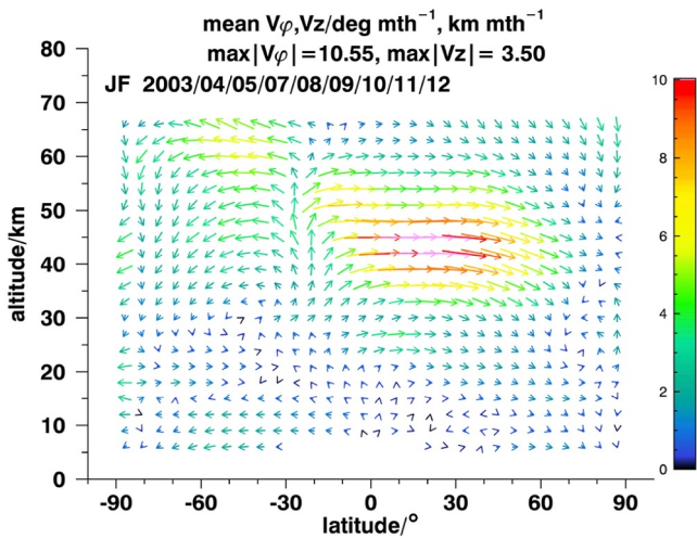
Figure 8. Mean monthly circulation pattern for January–February, derived from zonal mean distributions of the trace gases SF 6 , CFC-11, CFC-12, HCFC-22, CCl 4 , N 2 O, CH 4 , H 2 O, and CO, and the years given by the header, from MIPAS observations. Maximum velocities in meridional and vertical direction are also provided by the header. The color coding and length of the arrows is given by \sqrt{(\nu_\phi \text{ degree}^{-1} \text{ month})^2 + (\nu_z \text{ km}^{-1} \text{ month})^2} for \nu_\phi and \nu_z in units of degree per month and kilometer per month. Pink arrows refer to velocities higher than representable by the color scale chosen. For more details, see von Clarmann et al. (2021).
