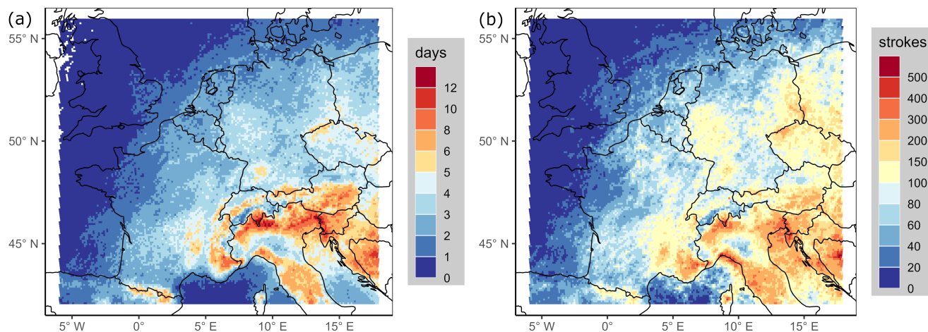
Figure 6. Mean annual number of (a) thunderstorm days (TDs) per 10 \times 10 \text{ km}^2 and (b) lightning density (strokes per 10 \times 10 \text{ km}^2 ; EUCLID, 2001–2021, MJJA).
