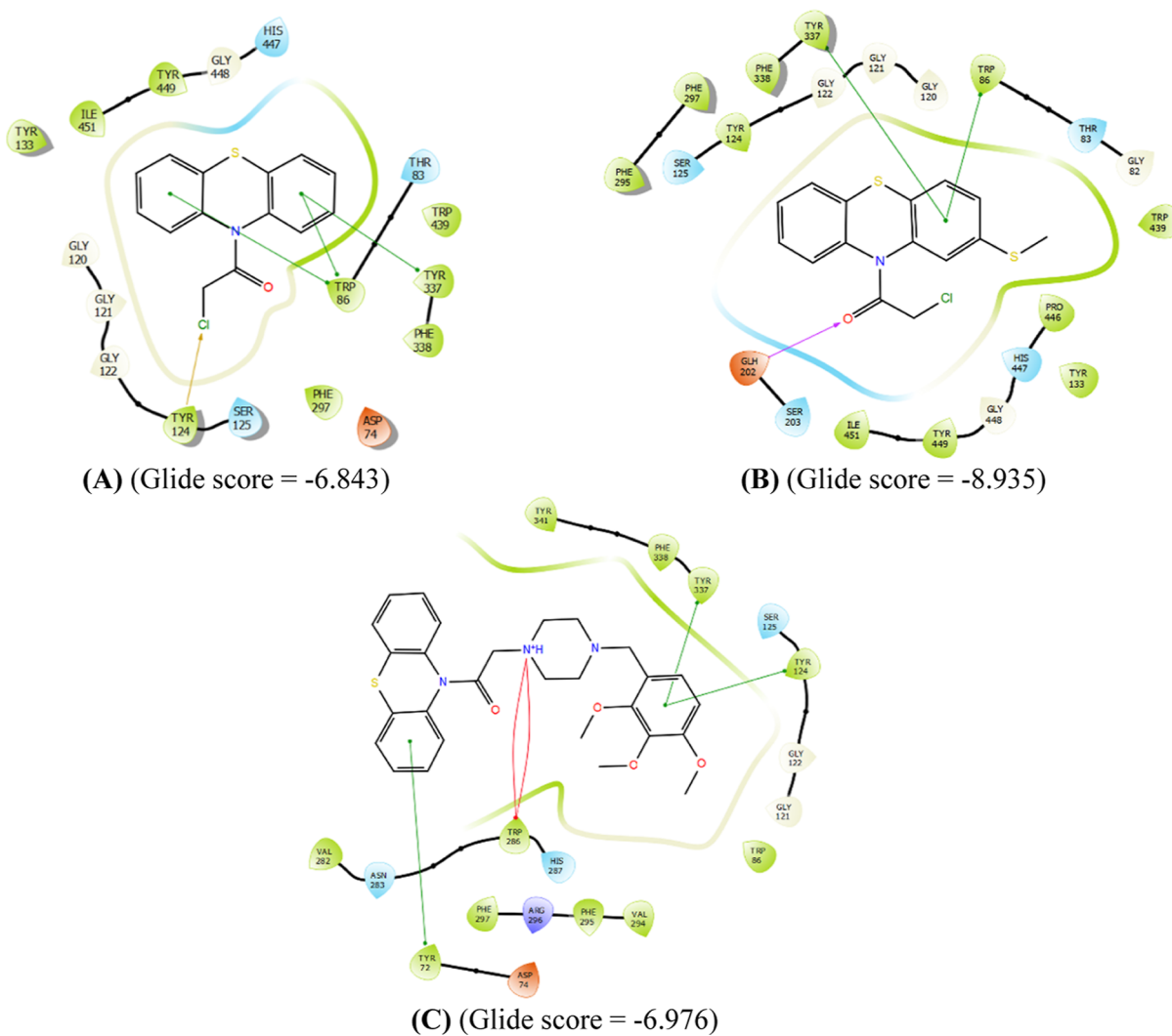
Figure 5. Interaction profiles of the most potent ligands 1 (A), 3 (B), and 8 (C) against HCC cell lines. Purple color represents H-bond interactions, whereas red elliptical line defines Pi-cation interaction. In addition, green lines represent Pi-Pi interactions, and gold arrow is for the halogen bond interaction.
