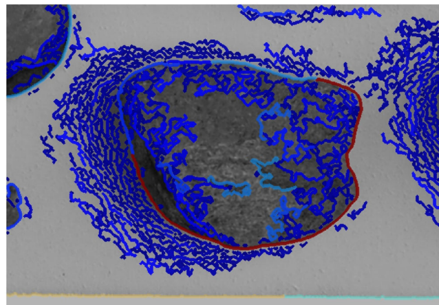
FIGURE 2 Connected components resulting from the application of the classical Canny segmentation algorithm. The red contour represents the longest connected component. Notice that, in the area where a shadow is present, on the left of the pebble, the algorithm identifies a series of possible edges, each with a different 'strength' and length.
