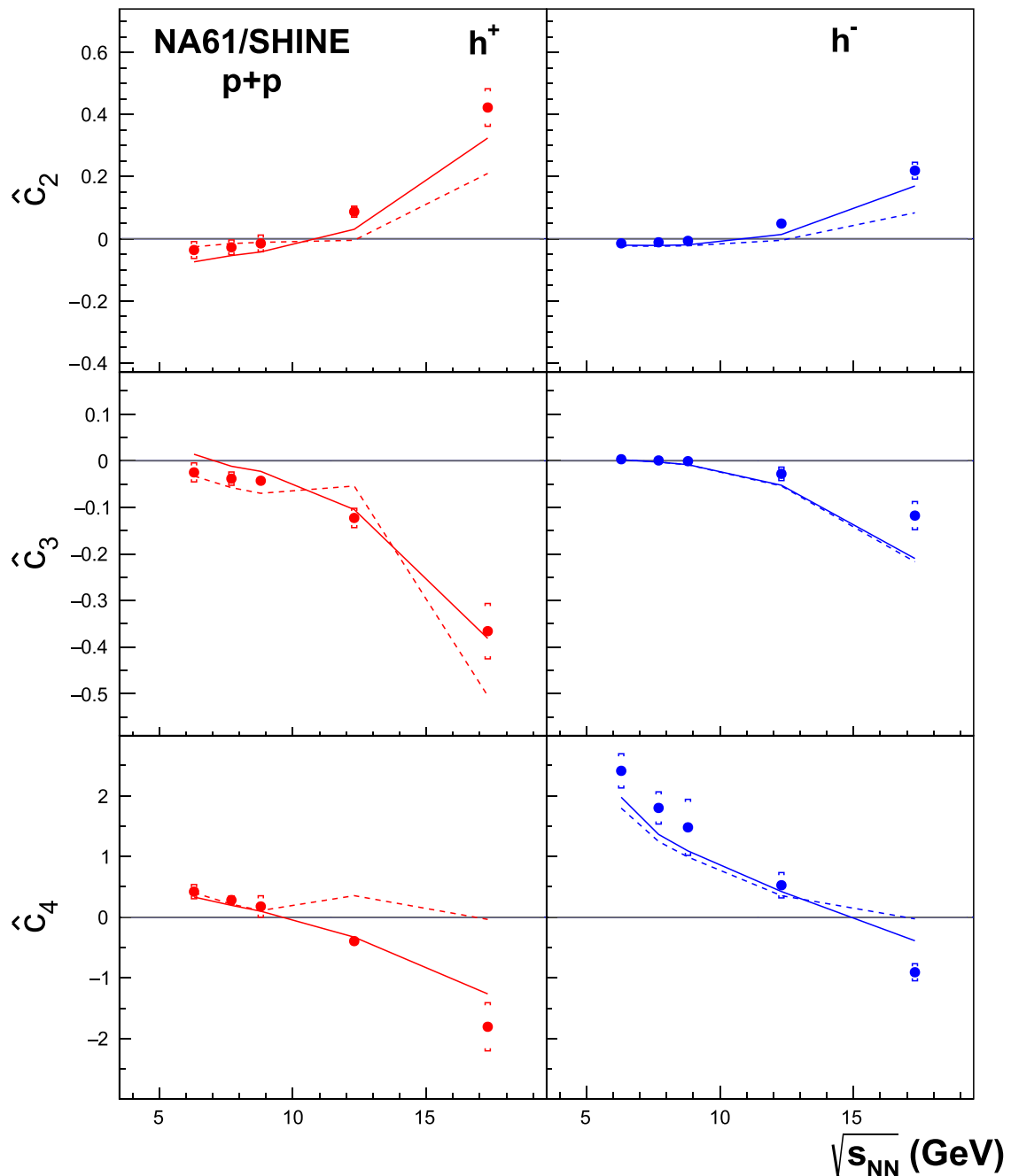
Fig. 7 Energy dependence of factorial cumulants of multiplicity distributions of h^+ and h^- in p+p interactions at \sqrt{s_{NN}} = 6.3, 7.7, 8.8, 12.3, and 17.3 GeV in the phase-space region as defined in Ref. [26]. The statistical uncertainty is indicated with a color bar (often smaller
