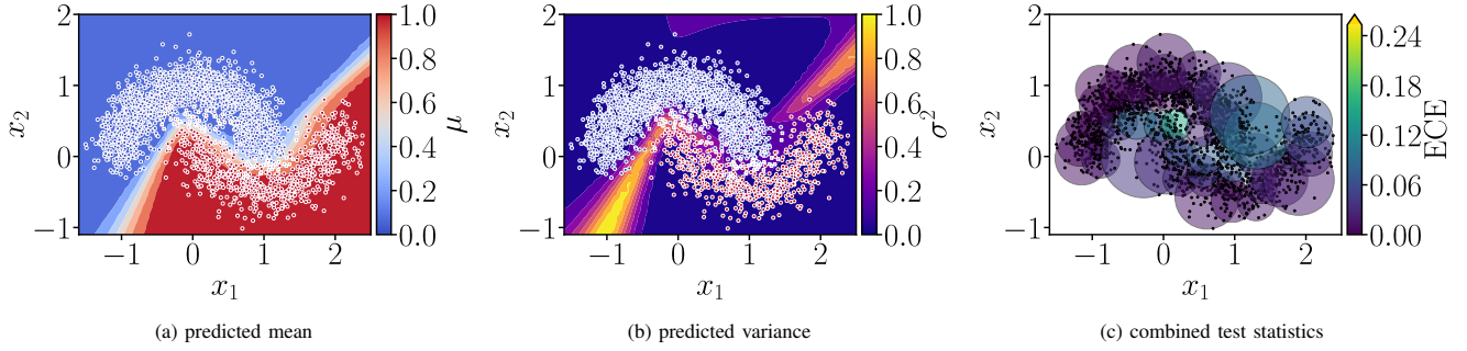
Fig. 4: Binary classification results with predicted mean (a) and variance (b), where dots mark the true classification of input test data and the incorrectly classified points are highlighted as crosses. The true labels are color-coded, with class label 0 displayed in blue and class label 1 in red. The combined test statistics per leaf node are displayed in (c).
