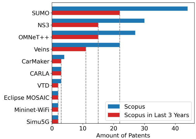
FIGURE 9. Reference numbers of the main V2X simulations found in security context in the Scopus database using the title, abstract, and keywords criteria.
