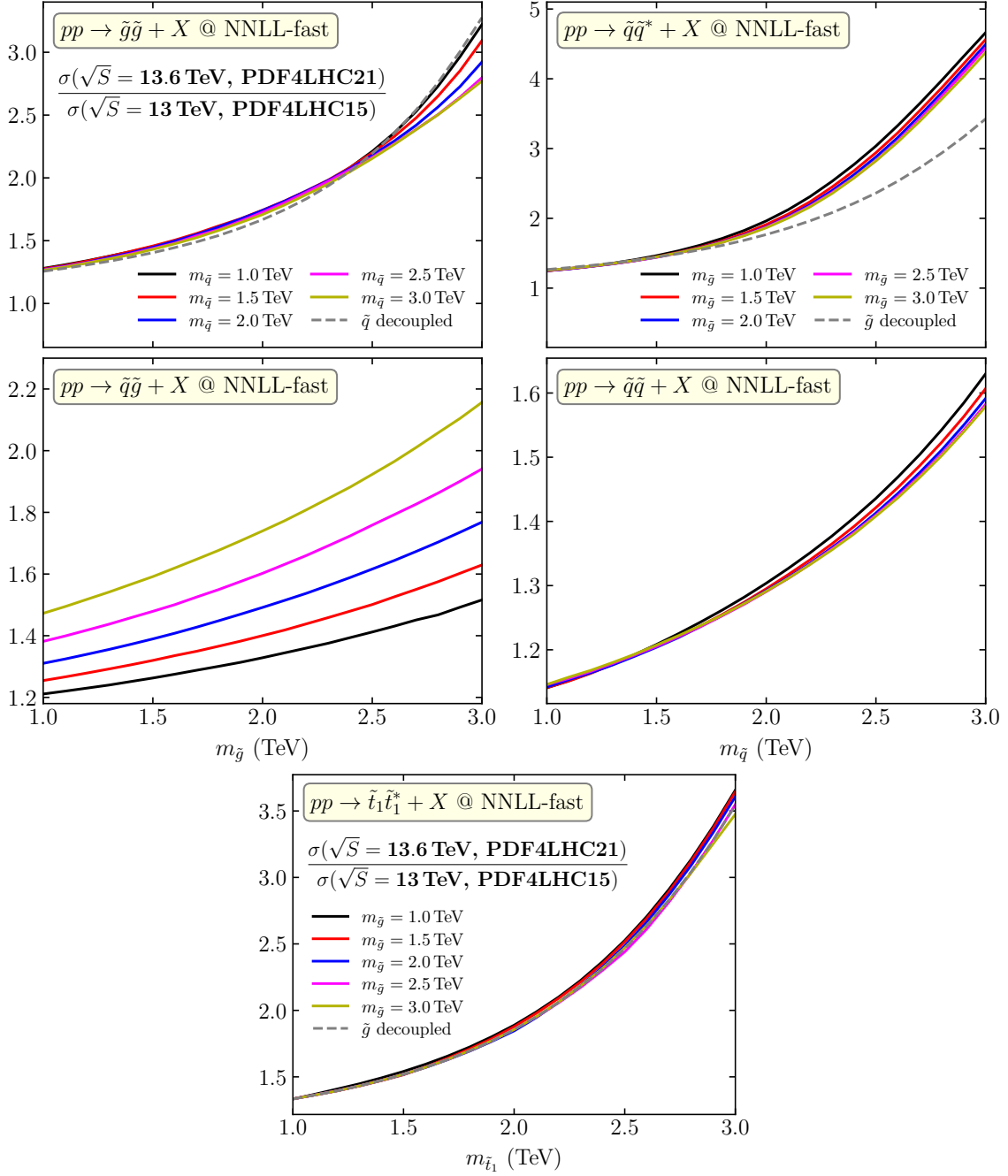
Figure 5: Comparison between the central \text{NNLO}_{\text{Approx}}+\text{NNLL} cross sections for squark, gluino, and stop production as provided by NNLL-FAST 2.0 (for \sqrt{S} = 13.6 \text{ TeV} and with PDF4LHC21) and the previous version NNLL-FAST 1.1 (for \sqrt{S} = 13 \text{ TeV} and with PDF4LHC15), presented as the ratio of the two. The ratios are shown depending on the mass of the produced sparticle for a range of values of the other mass parameter.
