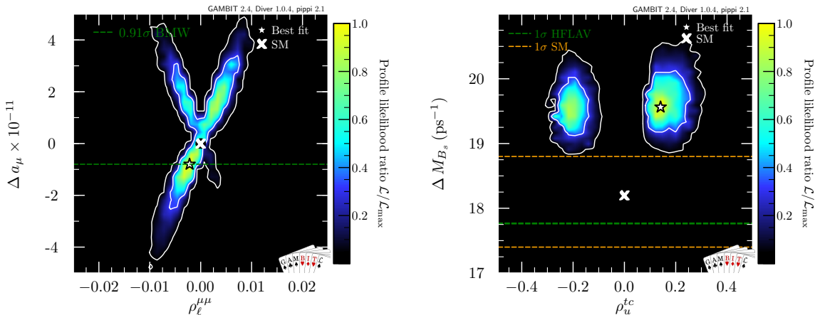
Figure 4: Profile likelihood ratios for \Delta a_\mu (left) and \Delta M_{B_s} (right) obtain from the full scan. As before the white star denotes the best-fit point and the white cross the SM prediction. White contours around the best fit point are the 1\sigma and 2\sigma confidence intervals.
