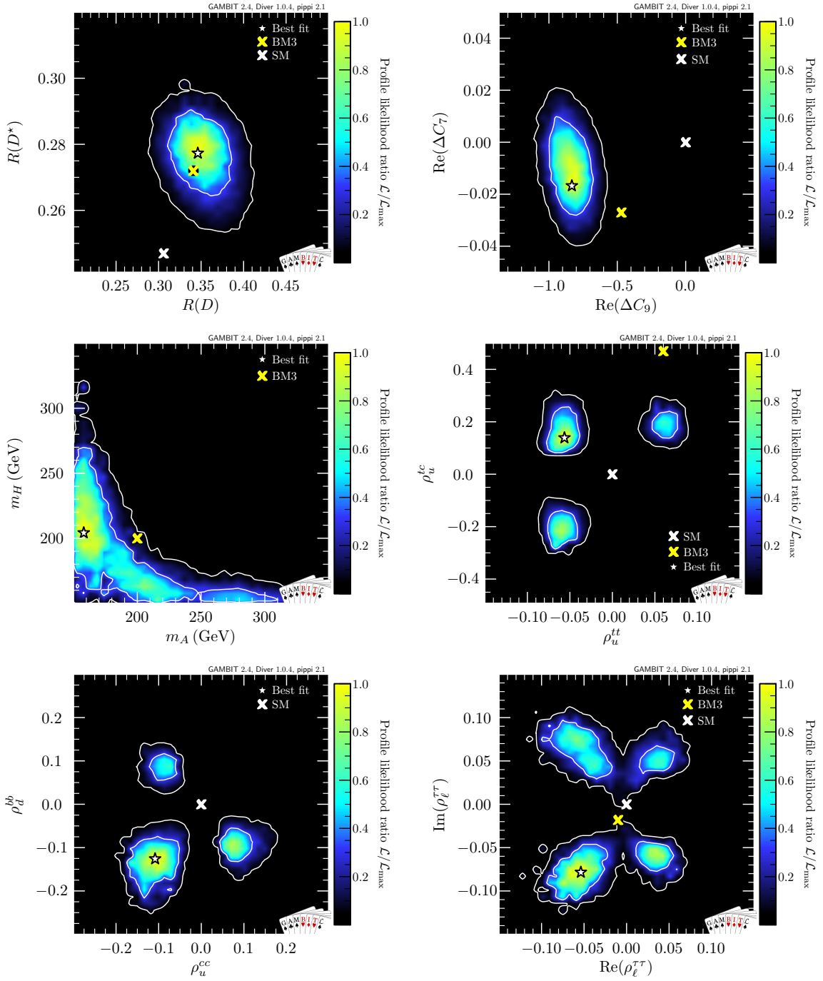
Figure 3: Profile likelihood ratio for different combinations of model parameters and observables for the full fit with the extended parameter set. As before the white star denotes the best-fit point, the white cross the SM prediction, and the yellow cross corresponds to BM3 from Ref. [24]. White contours around the best fit point are the 1\sigma and 2\sigma confidence intervals.
