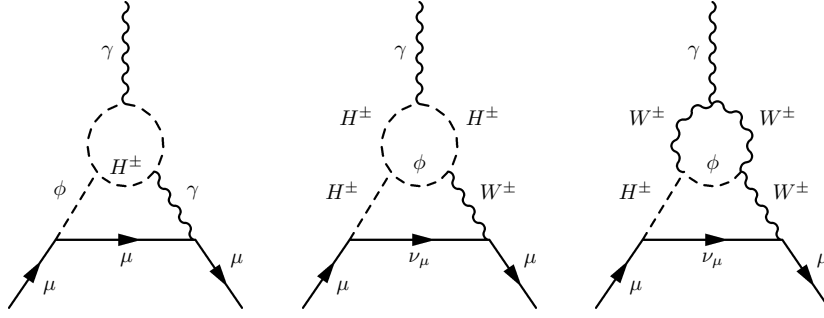
Figure 9: Two-loop bosonic Barr-Zee diagrams contributing to (g-2)_\mu . Here \phi = h, H, A , as in Figure 7. In the left panel, the internal photon \gamma may be replaced by a Z boson, and the internal H^\pm with a W^\pm boson.
