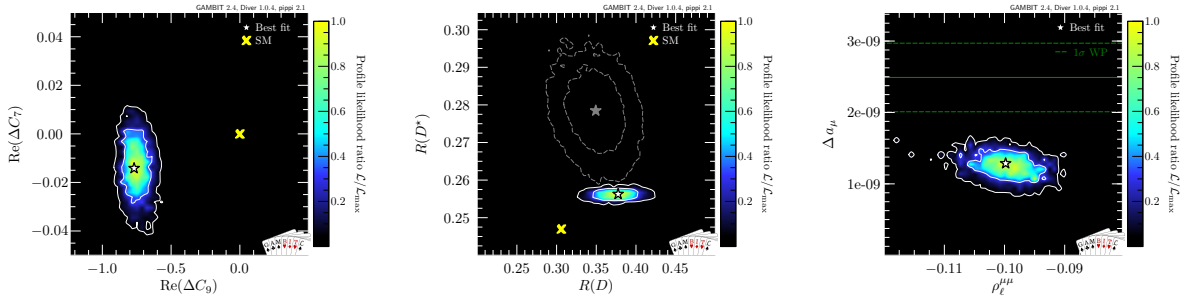
Figure 11: Profile likelihood ratios \mathcal{L}/\mathcal{L}_{max} for different 2D plots of the parameter space for the scan using the WP value for muon g-2 . The grey contours on the middle panel are the comparison with respect to the previous scan in section 4.
