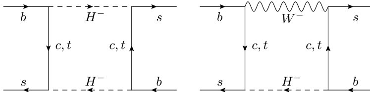
Figure 1: Box diagrams relevant for B_s - \overline{B}_s mixing.
