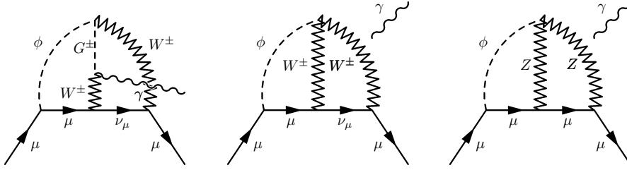
Figure 10: Two-loop bosonic 3 boson diagrams contributing to muon g-2 . Here \phi = h, H, A as in Figure 7. In the middle and right panels, the detached photon could be attached to either of the vector boson lines in the diagram. In the right panel, the scalar boson \phi may swap positions with the Z bosons.
