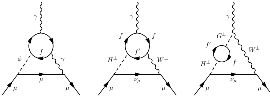
Figure 8: Two-loop fermionic Barr-Zee diagrams that contribute to (g-2)_\mu . The internal photon \gamma may be replaced by a Z boson, f' is the SU(2)_L partner of f and \phi = h, H, A .
