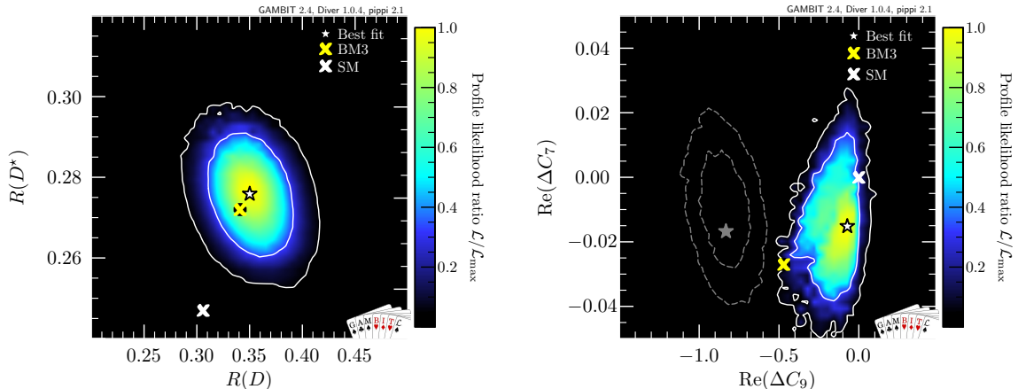
Figure 2: Profile likelihood ratios for R(D) and R(D^*) (left) and \Delta C_9 and \Delta C_7 (right). The white star denotes the best-fit point, the white cross the SM prediction, and the yellow cross corresponds to BM3 from Ref. [24]. White contours around the best-fit point are the 1\sigma and 2\sigma confidence intervals (calculated with two degrees of freedom). The grey contours on the right shows the region preferred by the model-independent fit to b \rightarrow s\ell^+\ell^- transitions.
