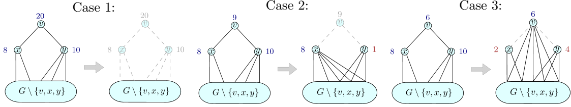
Figure 2: Illustration of the three cases of the Extended V-Shape Reduction.
