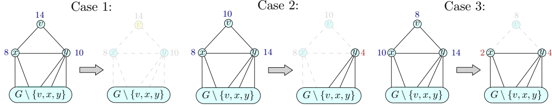
Figure 1: Illustration of the three cases of the Triangle Reduction.
