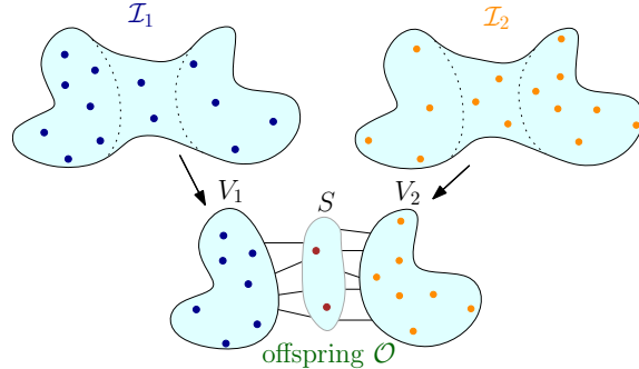
Figure 3: The vertex separator combine operation to create an offspring \mathcal{O} out of two individuals \mathcal{I}_1 and \mathcal{I}_2 .
