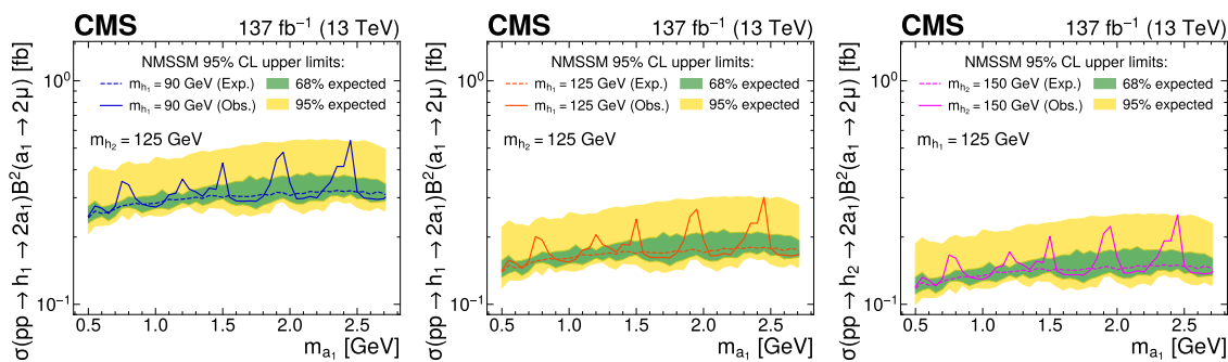
Figure 8. The 95% CL observed upper limits for \sigma(pp \rightarrow h_{1,2} \rightarrow 2a_1)\mathcal{B}^2(a_1 \rightarrow 2\mu) for the NMSSM as a function of m_{a_1} for three choices of m_{h_{1,2}} . The left and middle plots have m_{h_2} fixed to 125 GeV and the right plot has m_{h_1} fixed to 125 GeV. The data presented here reflect the results of the 2017 and 2018 data sets combined with the previously published results of the 2016 data set in [32].
