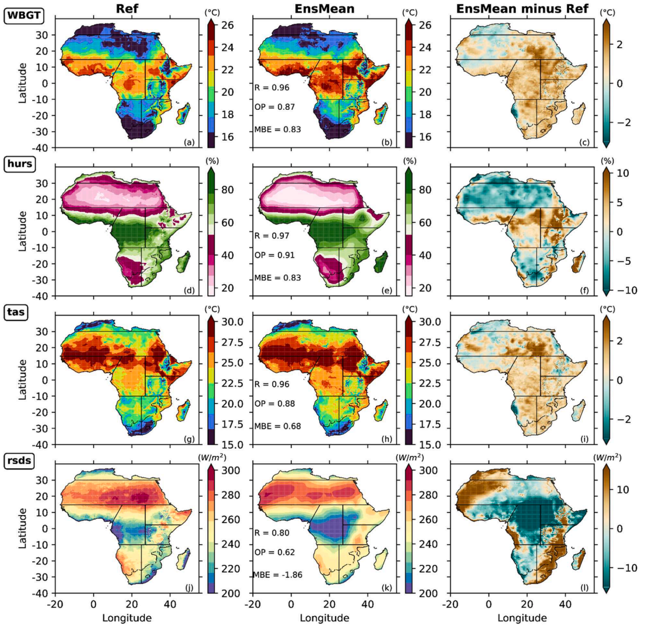
Fig. 2. Mean annual spatial distribution of the daily wet bulb globe temperature (WBGT), relative humidity ( hurs ), air temperature ( tas ), and shortwave radiation ( rsds ) for the reference data (Ref) and the multimodel ensemble mean of the NEX-GDDP-CMIP6 ( EnsMean ) with their bias ( EnsMean minus Ref ) in the present climate (1985–2014). Each row shows the variables, while the column indicates the name of the data. R indicates the spatial correlation. OP represents the overall spatial performance and the mean absolute error, respectively.
