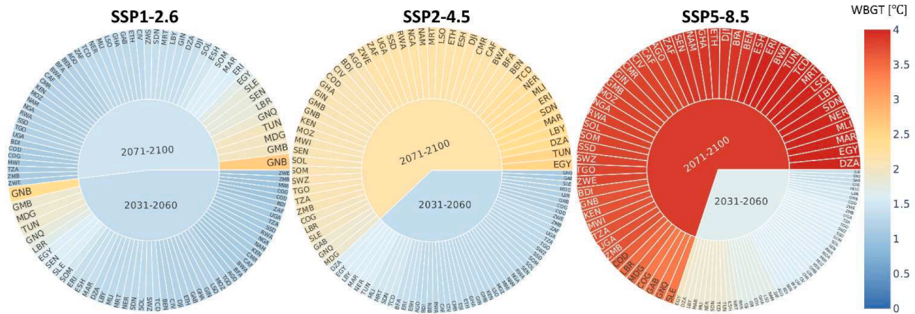
Fig. 6. 75th percentile projected changes in WBGT across countries under different climate scenarios and periods of the multimodel ensemble mean of the NEX-GDDP-CMIP6. The countries are ranked in ascending order for each period for a given scenario. The different colors of each country and period indicate the values depicted in the color bar.
