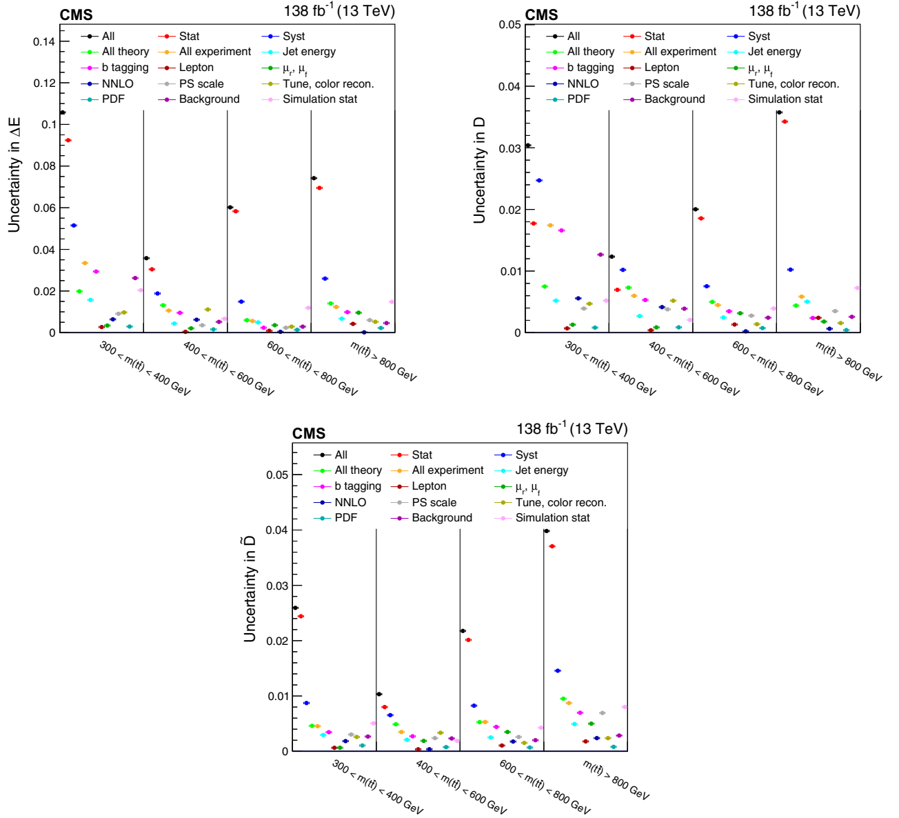
FIG. 24. Contribution of individual uncertainty sources or groups of uncertainties in the measured \Delta_E , D , and \tilde{D} in bins of m(t\bar{t}) .
