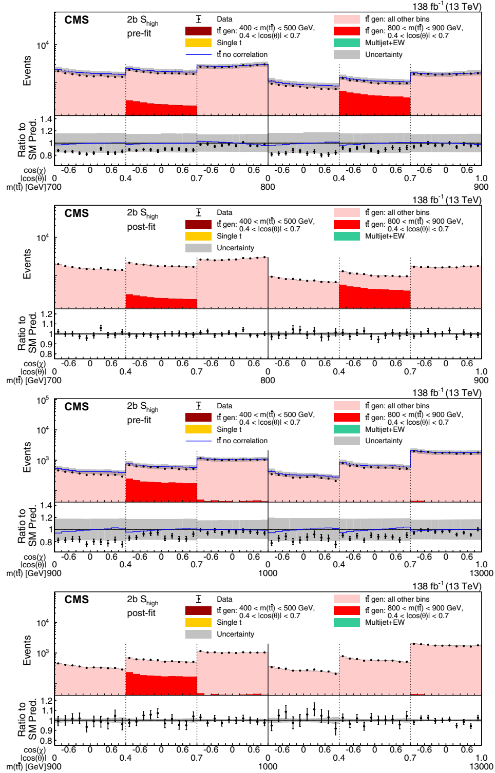
FIG. 14. Pre- and post-fit distributions of \cos(\chi) comparing the data (points) to the POWHEG+PYTHIA simulation (stacked histograms) for the D measurement in bins of m(t\bar{t}) vs |\cos(\theta)| in the 2b S_{\text{high}} category. The boundaries of the |\cos(\theta)| and m(t\bar{t}) bins are labeled and indicated by dashed and solid lines, respectively. For the illustration of resolution effects, t\bar{t} events generated in two selected m(t\bar{t}) vs |\cos(\theta)| bins are shown in different shades of red. All other t\bar{t} contributions are shown in pink. A model without any polarization and spin correlation is shown as a blue line. The gray uncertainty band indicates the combined statistical and systematic uncertainties in the prediction. The vertical bars on the points show the statistical uncertainty. Ratios to the predicted yields are provided in the lower panels.
