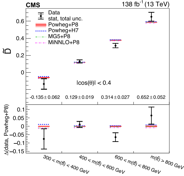
FIG. 27. Results of the \tilde{D} measurements in bins of m(t\bar{t}) for |\cos(\theta)| < 0.4 . The measurements (markers) are shown with the statistical uncertainty (inner error bars) and total uncertainty (outer error bars) and compared to the predictions of POWHEG+PYTHIA, POWHEG+Herwig, MadGraph5_aMC@NLO+PYTHIA and MiNNLO+PYTHIA. In the lower panel results are presented with the POWHEG+PYTHIA predictions subtracted. The POWHEG+PYTHIA prediction is displayed with ME scale and PDF uncertainties.
