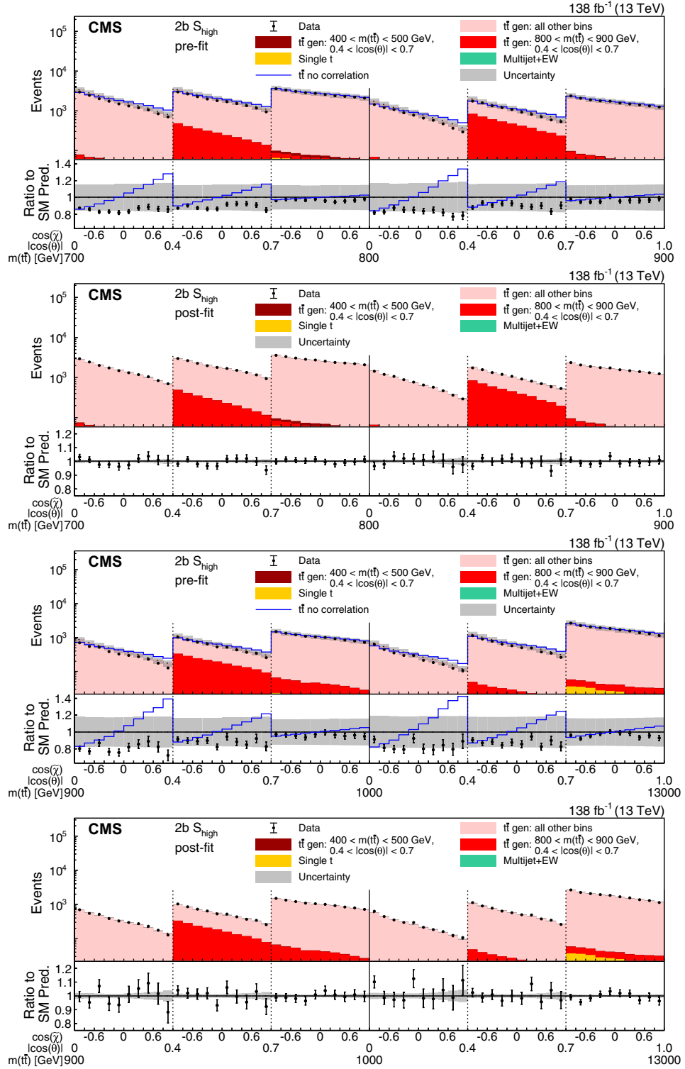
FIG. 16. Pre- and post-fit distributions of \cos(\tilde{\chi}) comparing the data (points) to the POWHEG+PYTHIA simulation (stacked histograms) for the \tilde{D} measurement in bins of m(t\bar{t}) vs |\cos(\theta)| in the 2b S_{\text{high}} category. The boundaries of the |\cos(\theta)| and m(t\bar{t}) bins are labeled and indicated by dashed and solid lines, respectively. For the illustration of resolution effects, t\bar{t} events generated in two selected m(t\bar{t}) vs |\cos(\theta)| bins are shown in different shades of red. All other t\bar{t} contributions are shown in pink. A model without any polarization and spin correlation is shown as a blue line. The gray uncertainty band indicates the combined statistical and systematic uncertainties in the prediction. The vertical bars on the points show the statistical uncertainty. Ratios to the predicted yields are provided in the lower panels.
