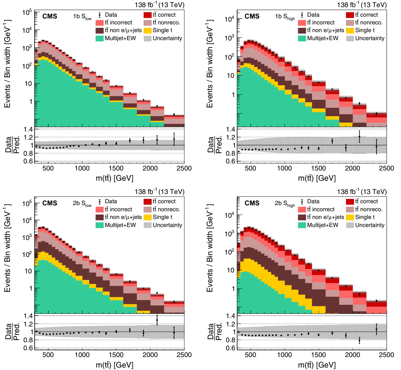
FIG. 4. Distribution of m(t\bar{t}) in all four categories. The data (points) are compared to the prediction (stacked histograms). The t\bar{t} and single top quark contributions are taken from the simulation, while the multijet + EW background is obtained from the CR. The t\bar{t} contribution is split into the correctly and incorrectly reconstructed, “nonreconstructable,” and non e/\mu + jets events. The gray uncertainty band indicates the combined statistical and systematic uncertainties in the prediction. The vertical bars on the points show the statistical uncertainty of the data. Ratios to the predicted yields are provided in the lower panels.
