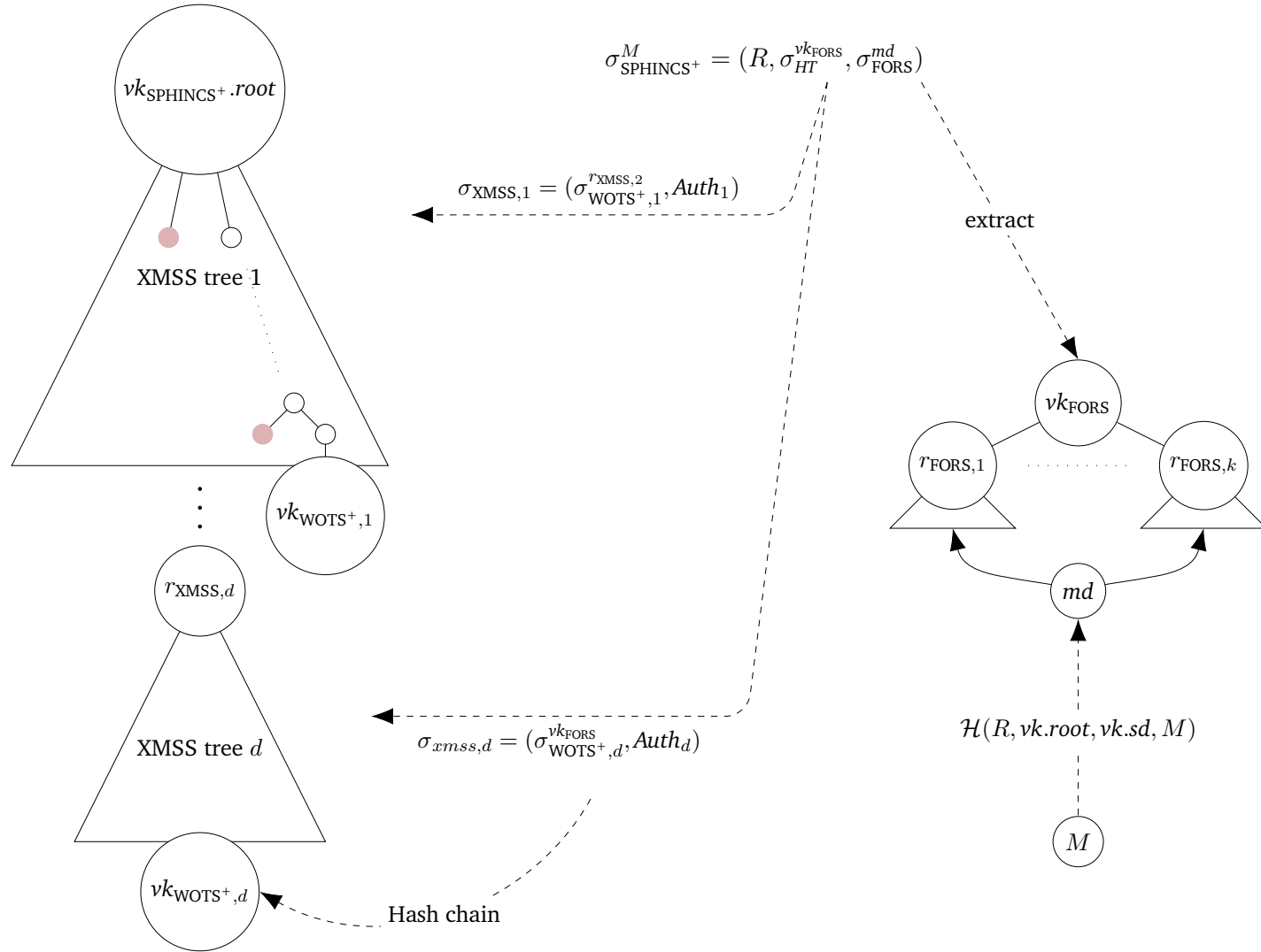
FIGURE 4.8: Overview of a SPHINCS + hypertree and a SPHINCS + signature \sigma_{\text{SPHINCS}^+}^M on message M . The signature consists of a random string R used to generate an initial message digest, a collection \sigma_{\text{HT}}^{vk_{\text{FORS}}} of XMSS signatures \sigma_{\text{XMSS}, i} , and a FORS signature. Each XMSS signature \sigma_{\text{XMSS}, i} consists of a WOTS + signature \sigma_{\text{WOTS}^+} and of an authentication path \text{Auth}_i , the latter of which contains the siblings of the nodes in the path from the XMSS leaf to the respective root. The leaf of each XMSS tree, vk_{\text{WOTS}^+} , can be computed from the signature \sigma_{\text{WOTS}^+}^{r_{\text{XMSS}, i+1}} by iterating the hash chain. The root of the FORS tree, vk_{\text{FORS}} , can be extracted from the FORS signature \sigma_{\text{FORS}}^M .
