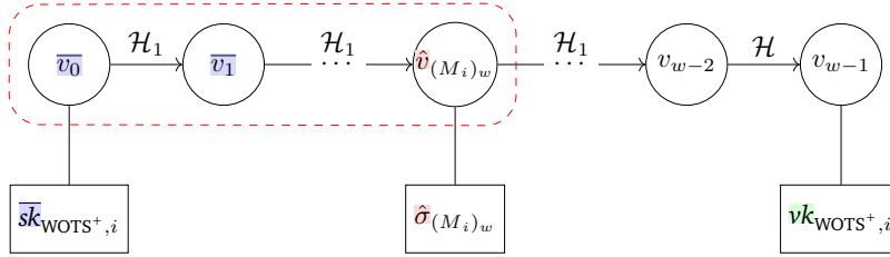
FIGURE 6.6: Simplified SPHINCS + scheme with the attacked part for the universal forgery for message \hat{M} in the dashed red box.
