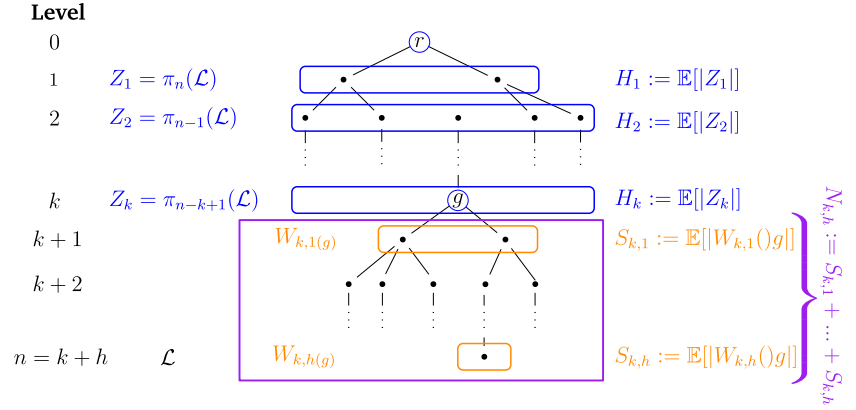
FIGURE 7.2: Combined classical-quantum enumeration tree. Quantum enumeration will happen on subtrees rooted at level k , here circled in purple.
