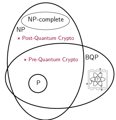
FIGURE 1.2: Placement of the power of quantum computing “BQP” in complexity theory. “Post-Quantum Crypto” refers to quantum-secure, “Pre-Quantum Crypto” to the conventional secure cryptosystems.
