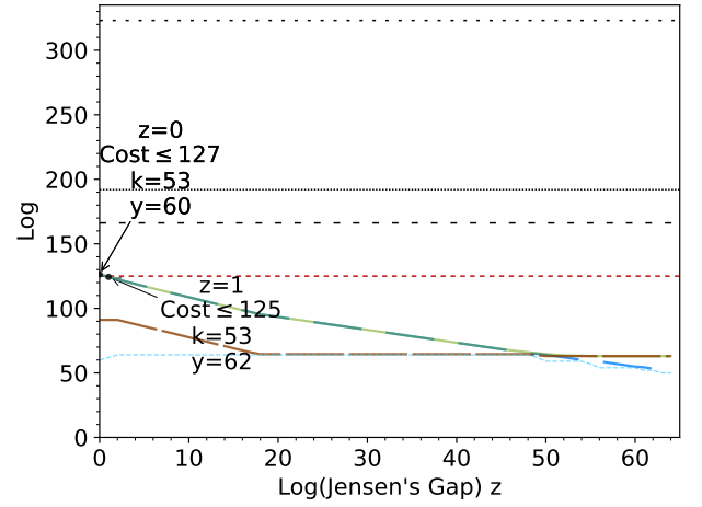
(c) Kyber-768, \text{MaxDepth} = 2^{96} .
