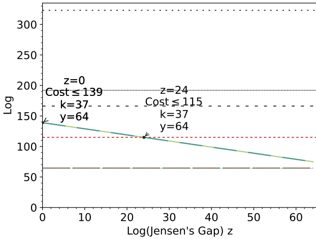
(b) Cost estimation for Kyber-768 w/ \text{MaxDepth} = \infty .
