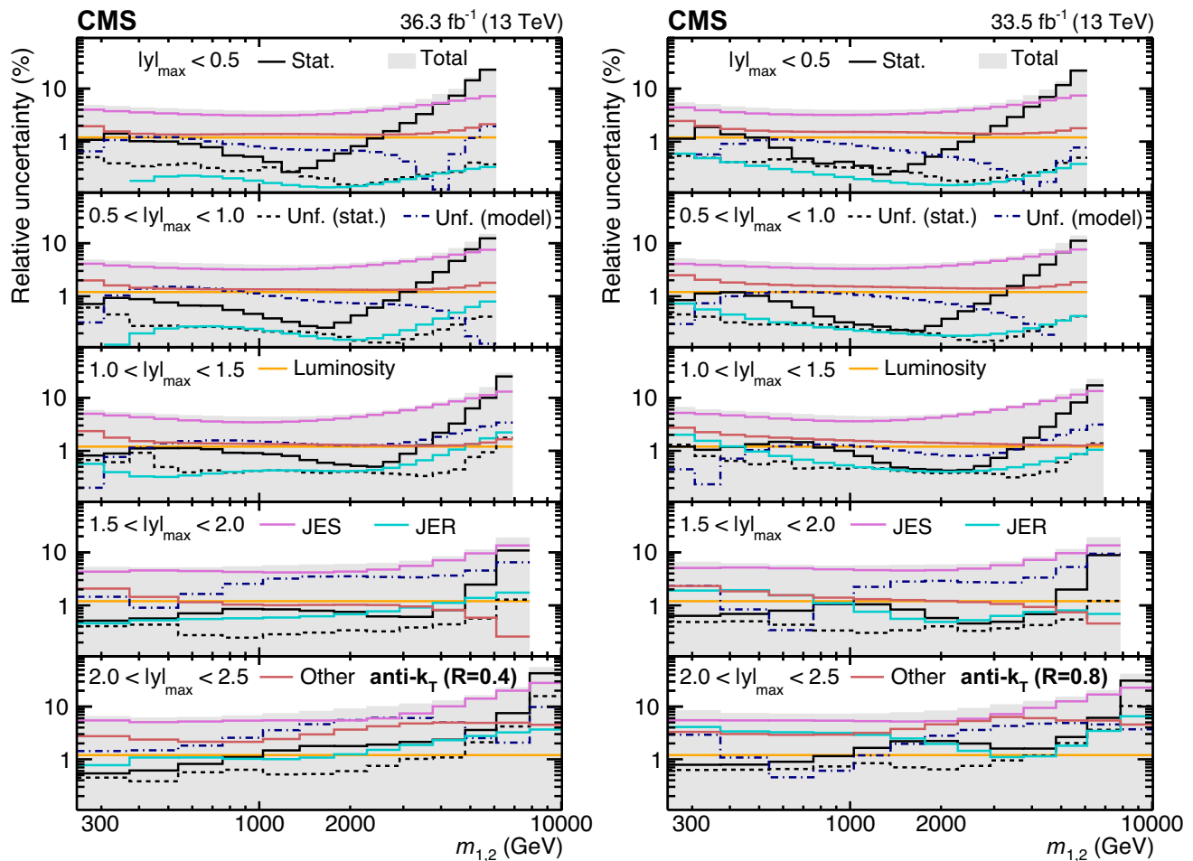
Fig. 3 Breakdown of the experimental uncertainty for the 2D measurements as a function of m_{1,2} using jets with R = 0.4 (left) and R = 0.8 (right). The individual components and abbreviations are explained in
