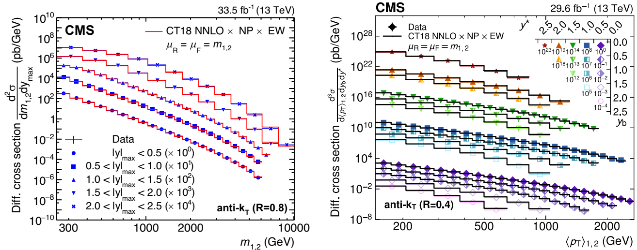
Fig. 8 Differential dijet cross sections, illustrated here for the 2D measurement as a function of m_{1,2} using jets with R = 0.8 (left), and the 3D measurement as a function of \langle p_{T,1,2} \rangle using jets with R = 0.4 (right). The markers and lines indicate the measured unfolded cross sections
