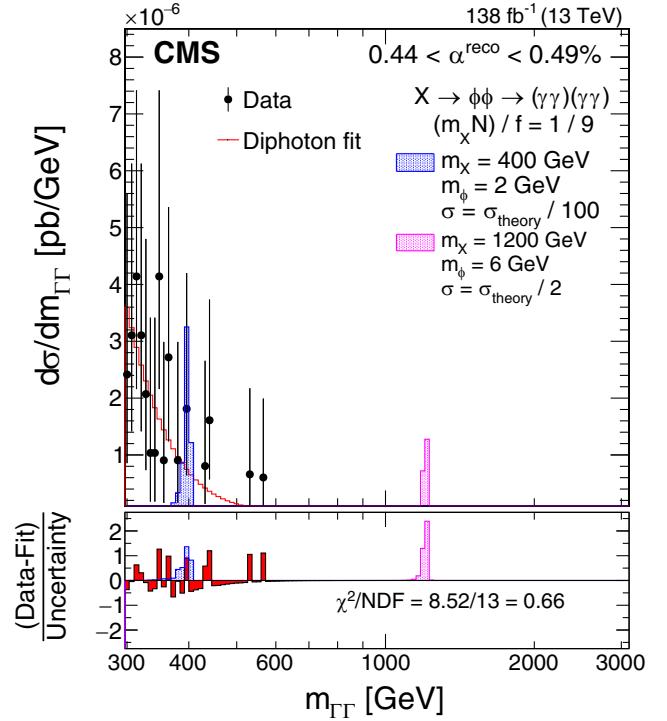
FIG. 2. Dicluster mass ( m_{T\Gamma} ) distribution for the data (points) for one of the \alpha^{\text{reco}} bins of the search ( 0.44 < \alpha^{\text{reco}} < 0.49\% ), fitted with the diphoton function (red), one of the considered five background parametrizations. Examples of two representative predicted signals are shown (blue and pink). The lower panel shows the difference between the observed data and the background prediction divided by the statistical uncertainty of the data ( \sigma_{\text{data}} ), the aforementioned signals divided by \sigma_{\text{data}} , and the goodness of fit measure \chi^2/\text{NDF} (where NDF is the number of degrees of freedom).
