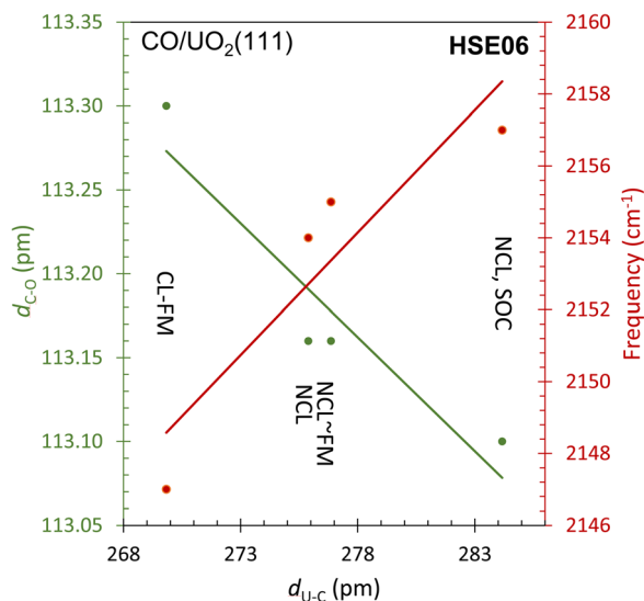
Fig. 9 A plot of the C to O bond distance ( d_{C-O} ) (left y-axis) and its frequency (right y-axis) as a function of the bond distance with the surface ( d_{U-C} ) as computed by HSE06 using the indicated methods. CL-FM: collinear ferromagnetic; NCL: non-collinear; SOC: spin-orbit coupling. The experimental \nu_{CO} frequency is equal to 2160\text{ cm}^{-1} .
