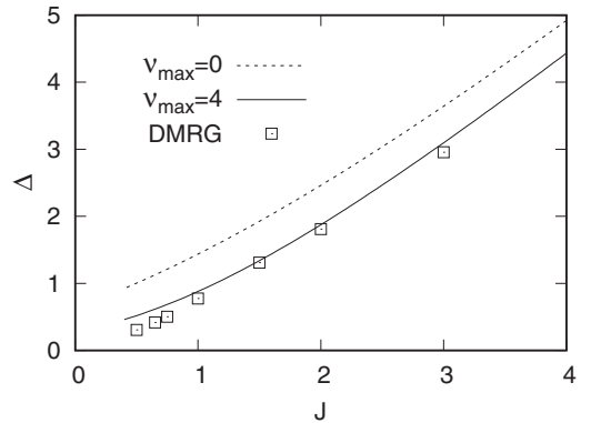
FIG. 8. Quasiparticle gap \Delta between k = 0 and \pi vs J for v_{\max} = 0 and 4 for the one-dimensional KLM compared to DMRG results by Yu and White [29] (DMRG).
