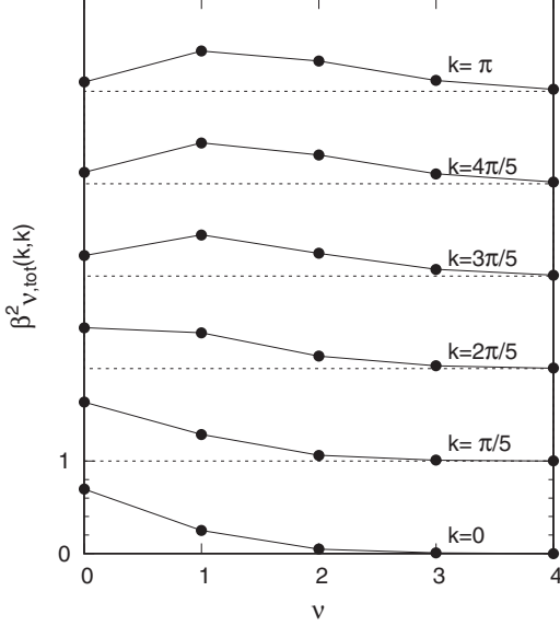
FIG. 3. Magnetic polaron wave function \beta_{v,\text{tot}}^2(k, k) for the lowest band for different k , J = 0.5 .
