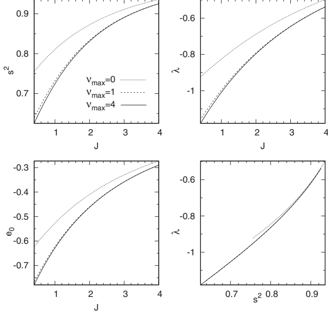
FIG. 5. The values of s^2 , \lambda , and the ground state energy per site, e_0 , vs J for different v_{\max} .
