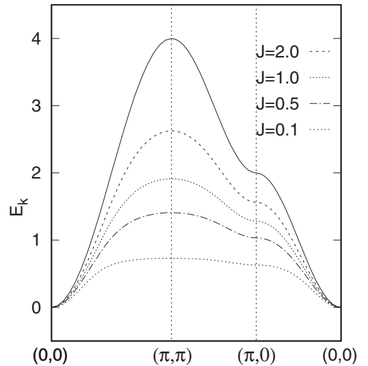
FIG. 2. Dispersion E_{\mathbf{k}} (in units of t ) for a single b^\dagger fermion for different J (dashed lines) compared to the unrenormalized band structure \frac{3J}{4} + \frac{\epsilon_{\mathbf{k}}}{2} (full line). A J -dependent constant has been subtracted from all bands to align them at \mathbf{k} = (0, 0) .
