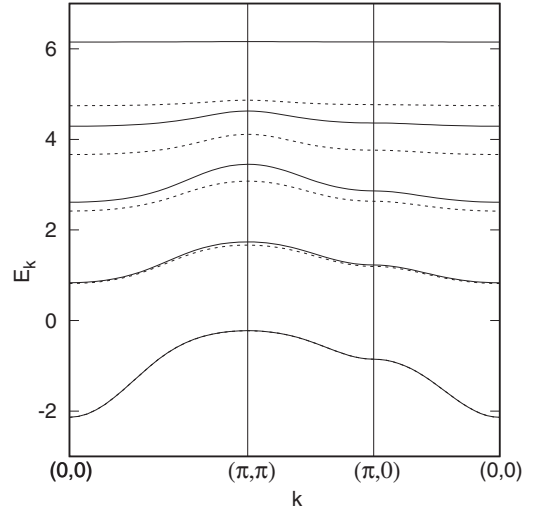
FIG. 1. Band dispersion E_{\mathbf{k}} (in units of t ) for a single b^\dagger fermion, J = 1 . The figure compares results for \nu_{\max} = 4 (full line) and \nu_{\max} = 8 (dotted line).
