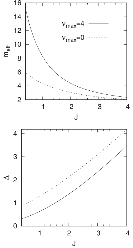
FIG. 7. Effective mass m_{\text{eff}} for the heavy part of the band structure at (\pi, \pi) and quasiparticle gap \Delta between \mathbf{k} = (0, 0) and (\pi, \pi) vs J for v_{\max} = 0 and 4.
