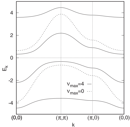
FIG. 6. Band structure for J = 1 for v_{\max} = 0 and 4. For v_{\max} = 4 only four of the ten bands are shown.
