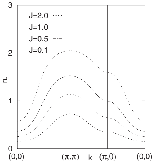
FIG. 4. Triplet content n_t for the lowest magnetic polaron state of a single b^\dagger fermion as a function of wave vector \mathbf{k} .
