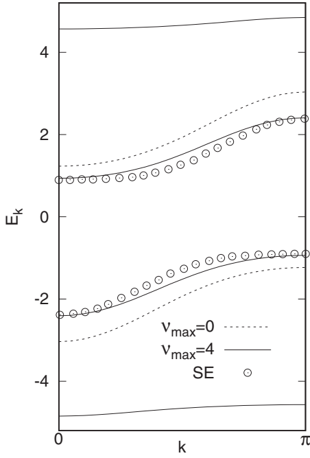
FIG. 9. Band structure at J = 2 for the one-dimensional KLM from the present theory compared to the series expansion result by Trebst et al. [42] (SE).
