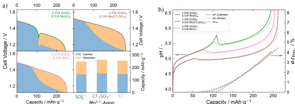
Fig. 10. a) Galvanostatic discharge behavior at 200\text{mA g}^{-1} for a 2\text{M ZnSO}_4 electrolytes with different Mn-salts added. Shown are the simulated cell voltages during the discharge in the second cycle. The colored areas below the discharge potential represent the fractional contribution of the \text{Zn}^{2+} -insertion current and the \text{Mn}^{2+} -dissolution current. The axis on the lower right shows the cumulative capacities of the insertion and dissolution process during discharge. b) Evolution of pH at the electrodes and for the tested electrolytes. The electrolyte pH at both anode and cathode and the average volume-fraction of Zinc-salt precipitate in the cell are shown.
