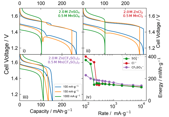
Fig. 9. i)-iii) Galvanostatic cycling behavior for discharge rates between 100\text{mA g}^{-1} and 10\text{A g}^{-1} in sulfate, chloride and triflate-based ternary electrolytes. iv) Comparison of the discharged energy content as a function of discharge current.
