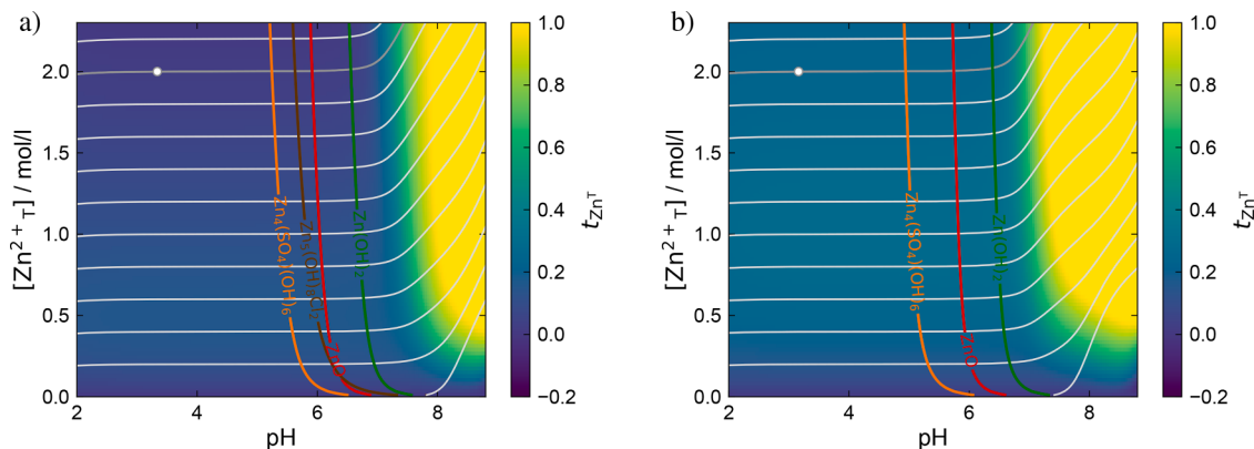
Fig. 6. Solubility Limits and Zn-Transference numbers of the quaternary electrolytes. Shown are the results for \text{ZnSO}_4 with an a) 0.5M \text{MnCl}_2 additive, and b) a 0.5M \text{Mn}(\text{CF}_3\text{SO}_3)_2 additive for a given total zinc concentration and electrolyte pH. The colored lines indicate the solubility limits of all relevant precipitation reactions.
