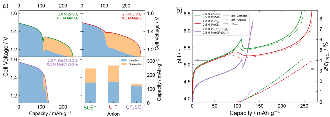
Fig. 8. a) Galvanostatic discharge behavior at 200\text{mA g}^{-1} (equal to 0.4\text{mA cm}^{-2} at the simulated mass loading of 2\text{mg cm}^{-2} ) for different ternary electrolytes. Shown are the simulated cell voltages during the discharge. The colored areas below the discharge potential represent the fractional contribution of the \text{Zn}^{2+} -insertion current and \text{Mn}^{2+} -dissolution current to the overall cell current. b) Evolution of pH at the electrodes during discharge. The electrolyte pH at both anode and cathode and the average volume-fraction of zinc-salt precipitate in the cell are shown.
