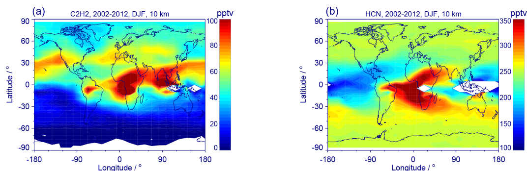
Figure A1. Global distributions of (a) \text{C}_2\text{H}_2 and (b) \text{HCN} measured by MIPAS at 10 km altitude during December to February, averaged over the time period 2002 to 2012. White areas: no data due to cloud filter.
