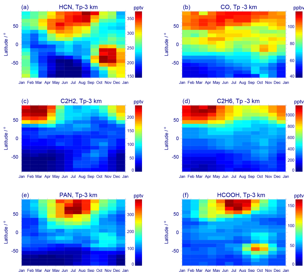
Figure 6. Time series of monthly composites of (a) HCN, (b) CO, (c) C_2H_2 , (d) C_2H_6 , (e) PAN, and (f) HCOOH VMRs in 10^\circ -wide latitude bands at an altitude of 3 km below the tropopause. The datasets are averaged over the time period 2002–2012.
