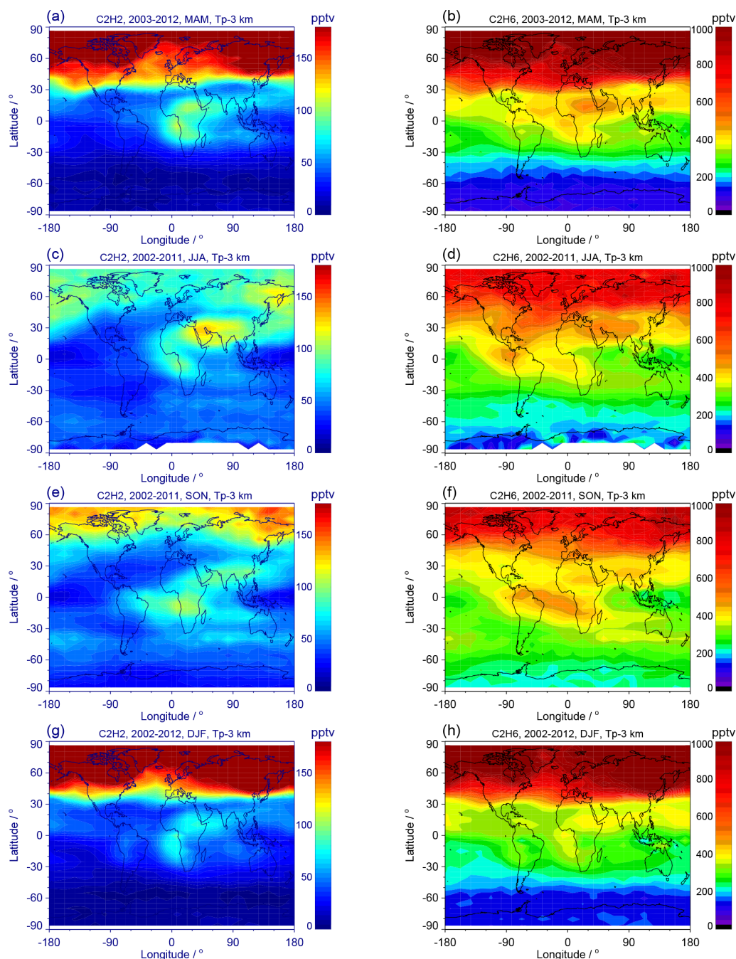
Figure 4. Global \text{C}_2\text{H}_2 distribution measured by MIPAS at 3 km below the tropopause during (a) March to May, (c) June to August, (e) September to November, and (g) December to February, as well as global \text{C}_2\text{H}_6 distribution measured by MIPAS at 3 km below the tropopause during (b) March to May, (d) June to August, (f) September to November, and (h) December to February. The distributions are averaged over the time period 2002 to 2012.
