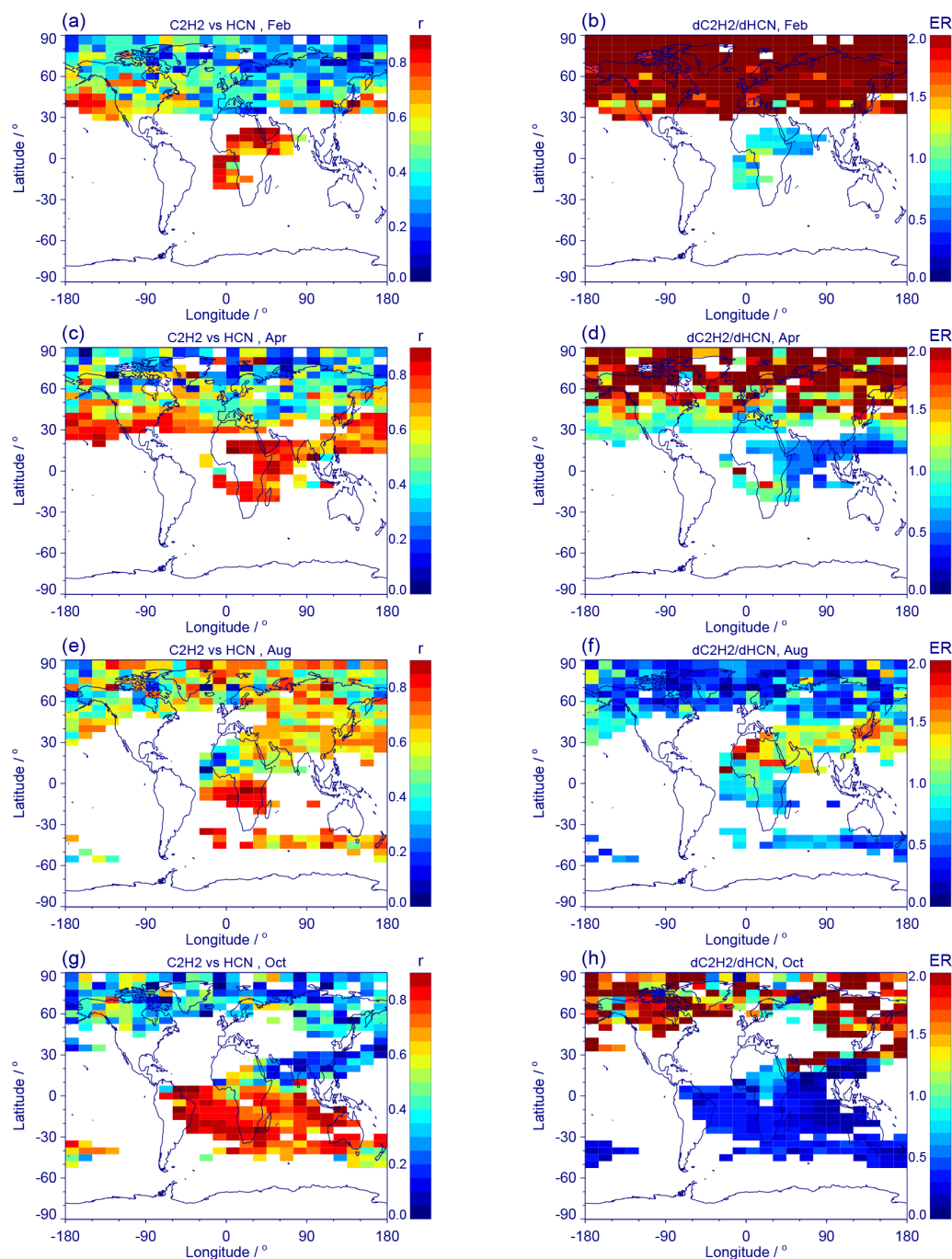
Figure 10. Global distribution of correlation coefficients r between MIPAS measurements of \text{C}_2\text{H}_2 and HCN in the upper troposphere for (a) February, (c) April, (e) August, and (g) October, as well as the respective \Delta\text{C}_2\text{H}_2/\Delta\text{HCN} enhancement ratios (ERs) in \text{pptv pptv}^{-1} for (b) February, (d) April, (f) August, and (h) October. White areas are regions with correlation coefficients or enhancement ratios lower than zero, with \text{C}_2\text{H}_2 VMRs lower than 60 pptv, or with bins containing fewer than 10 values. For further details, see Fig. 9.
