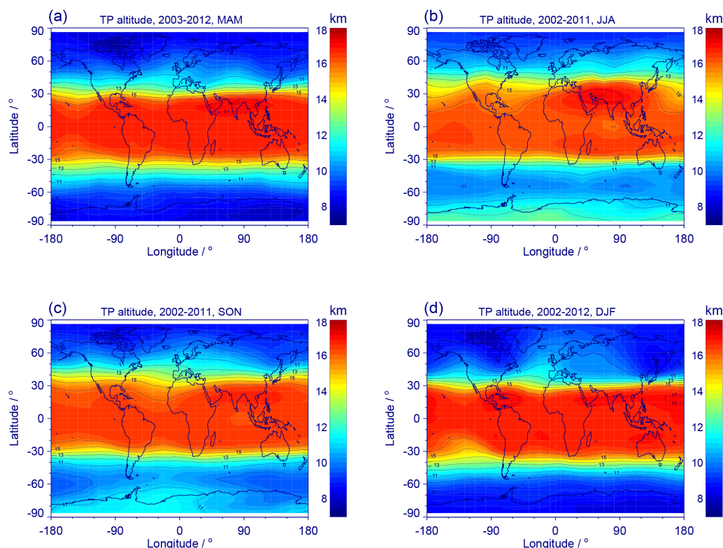
Figure 1. Global distribution of the thermal tropopause derived from MIPAS temperature profiles for the periods (a) March to May, (b) June to August, (c) September to November, and (d) December to February. The data are bin averages ( 5^{\circ} \times 15^{\circ} latitude by longitude, 7.5^{\circ} \times 15^{\circ} latitude by longitude at the poles) of the time period 2002 to 2012.
