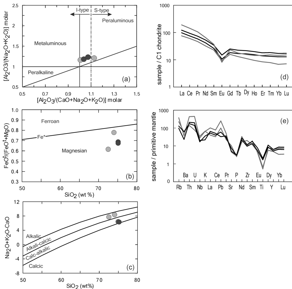
Fig. 6 Various classification diagrams for granites based on a–c major elements, d–e trace elements (black dots: granitoids GK7, GK8, grey dots: granophyre granites GK2, GK5). a Shand index plot with discrimination fields after Maniar and Piccoli (1989). The dividing line between I- and S-type granites is after Chappell and White (1974). b \text{FeO}^{\text{I}}/(\text{FeO}^{\text{I}} + \text{MgO}) versus \text{SiO}_2 (wt%) classification diagram (Frost et al. 2001). The Fe-number ( \text{Fe}^* ) dividing line is after
