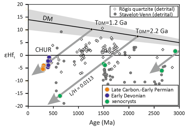
Fig. 9 Age versus \epsilon\text{Hf}_i diagram showing the results of Lu–Hf isotope analyses of zircon grains from Bode dike xenoliths (red, blue, green circles). Data from the Stavelot–Venn Massif (Willner et al. 2013) and the Ruhla Crystalline Complex (Rögis quartzite: Zeh and Gerdes 2010) are shown for comparison. CHUR- chondritic uniform reservoir, DM- depleted mantle evolution, L/H = ^{176}\text{Lu}/^{177}\text{Hf} = 0.0113, grey arrow—crust evolutionary trend. T_{\text{DM}} —two-stage Hf model age
