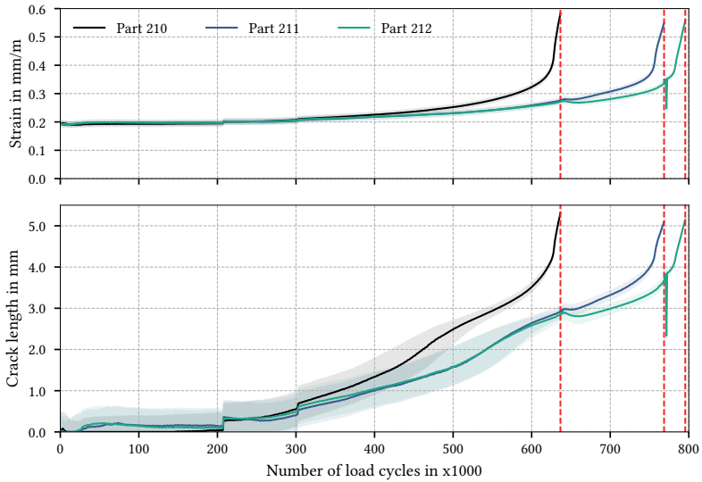
Figure 5.27: Maximal floating strain measured at channel two and corresponding estimated characteristic crack lengths of specimens 210-212 with the semi-transparent confidence area for a strain error of \Delta\epsilon = \pm 10 \mu\text{m}/\text{m} .
