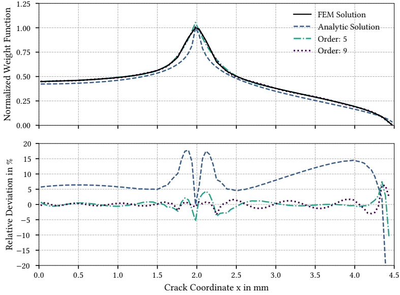
Figure 4.8: FEM Solution of the weight function and piecewise polynomial regressions of various order for a pressure strip at \xi_t = 2.0 \text{ mm} .
