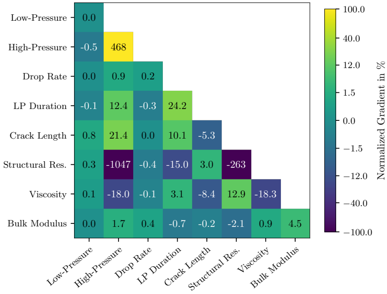
Figure 6.6: Heatmap of the median of the absolute gradients of the estimated crack propagation rate da/dN , normalized to 100% (main diagonal: gradient along primary parameter, lower triangular matrix: second gradient along primary and secondary parameter).
