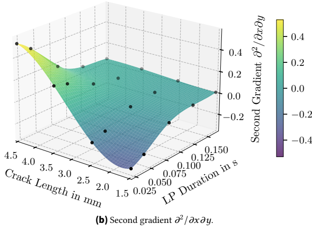
Figure 6.5: Influence of duration of the low-pressure (LP) phase and crack length on the SIF amplitude.
