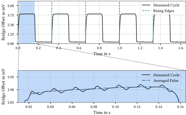
Figure 5.16: Cyclic average filter with rising edges separating the individual pulses and magnification of the averaged pulse of this cycle.
