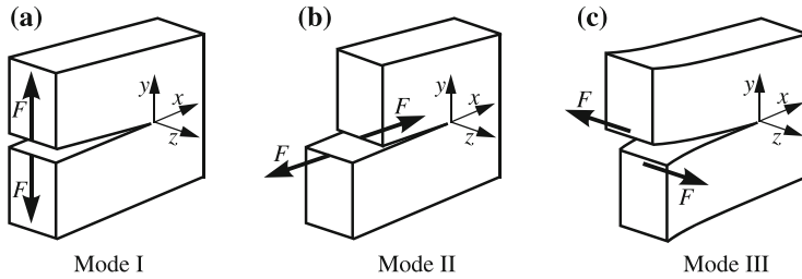
Figure 2.1: Crack opening modes, [13].
