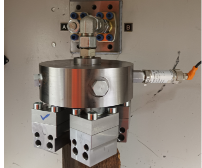
(b) Picture of the mounted test assembly inside the test chamber of the hydraulic test rig.
