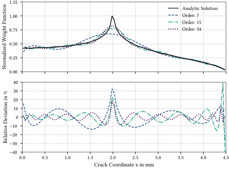
Figure 4.7: Analytic solution of the weight function for infinite elastic plates and polynomial regressions of various orders for a pressure strip at \xi_l = 2.0 \text{ mm} .
