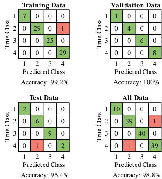
Figure 7. CNN performance accuracy for 4-class classification
